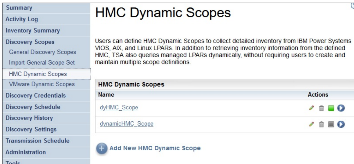
Figure 62. HMC Dynamic Scopes
