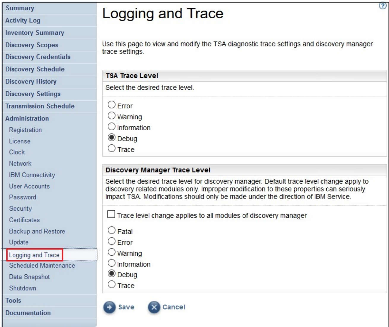
Figure 85. Logging and Trace
