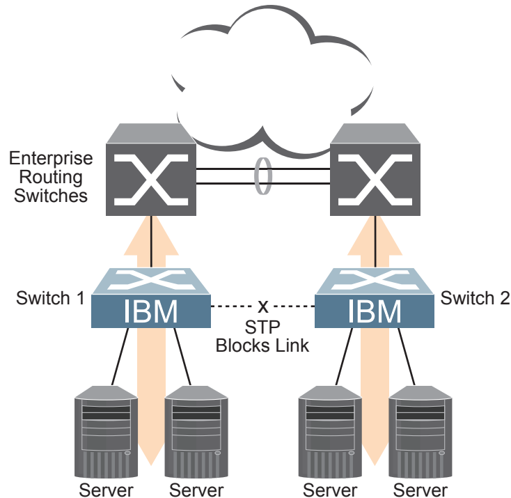
Figure 12. Spanning Tree Blocking a Switch-to-Switch Link
