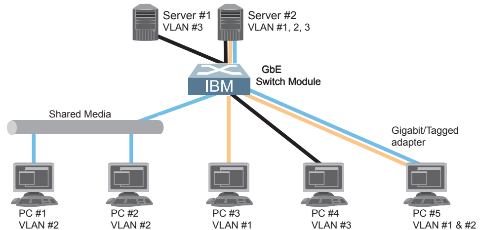
Figure 9. Multiple VLANs with VLAN-Tagged Gigabit Adapters
