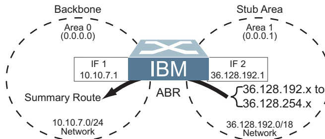
Figure 45. Summarizing Routes
