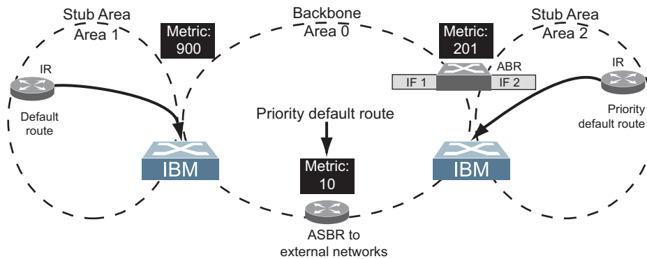
Figure 41. Injecting Default Routes
