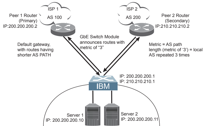
Figure 37. BGP Failover Configuration Example
