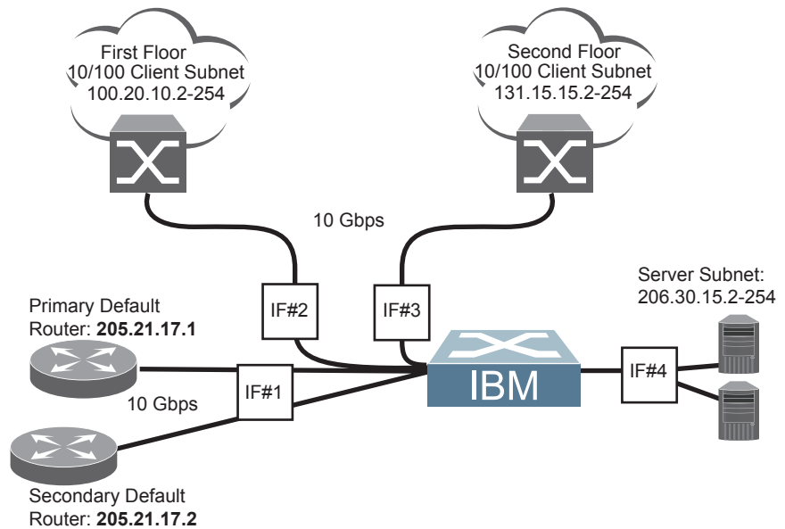
Figure 30. Switch-Based Routing Topology
