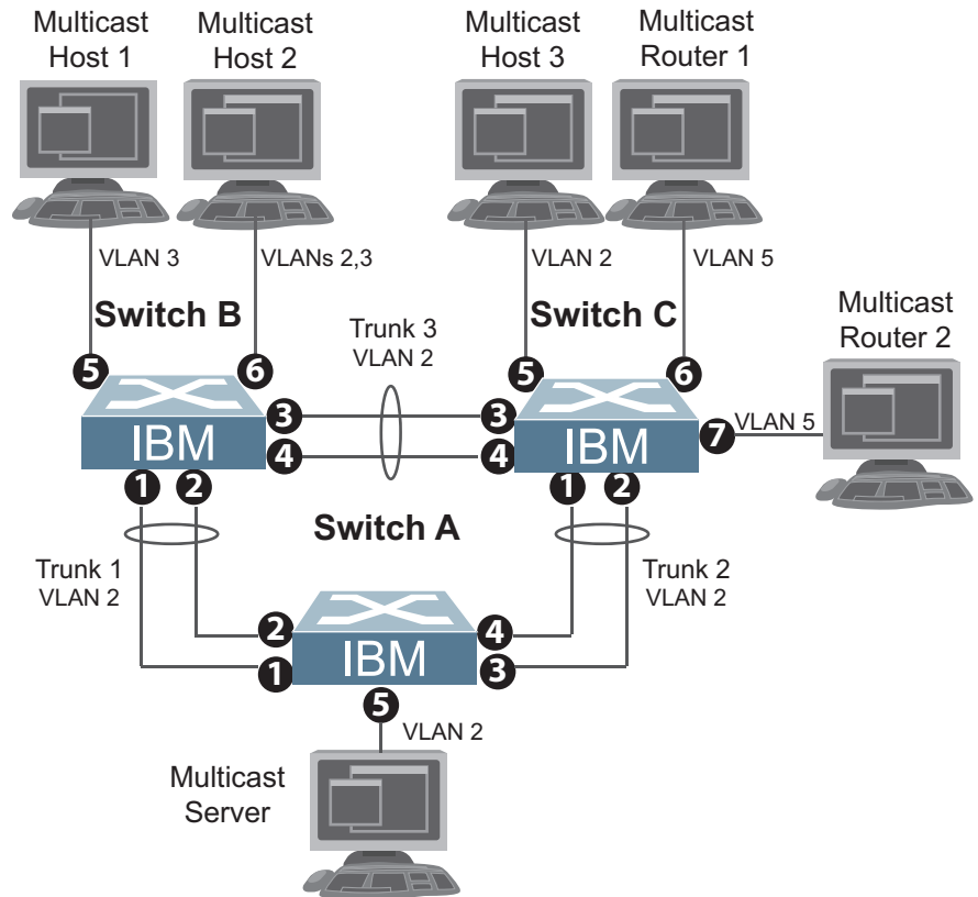
Figure 34. Topology
