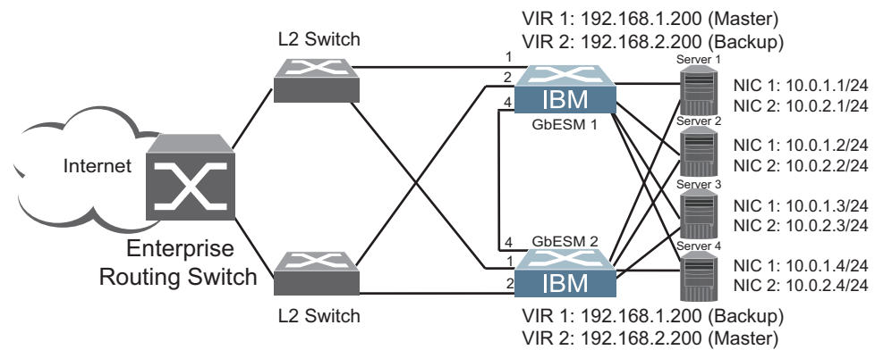
Figure 56. Active-Active High-Availability Configuration
