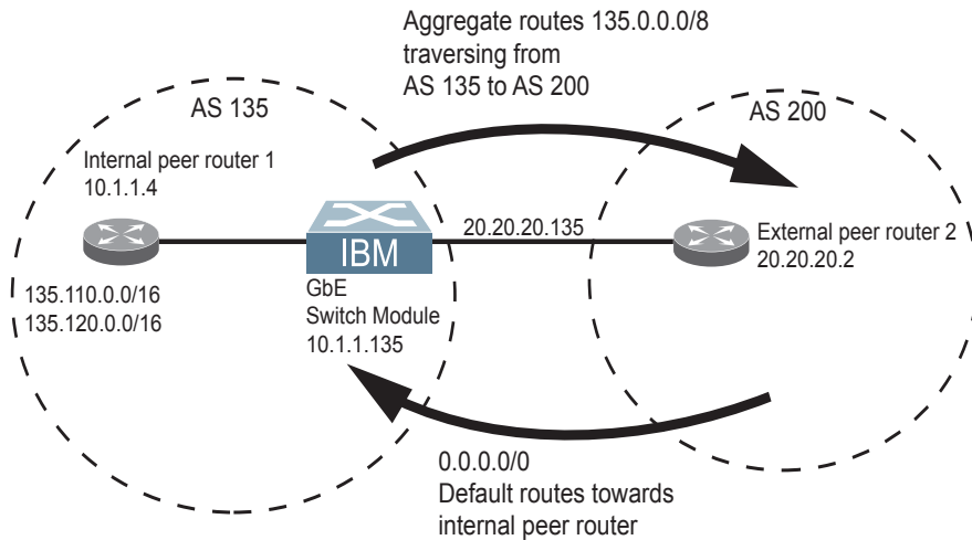
Figure 38. Route Aggregation and Default Route Redistribution
