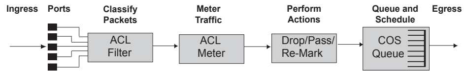
Figure 17. QoS Model
