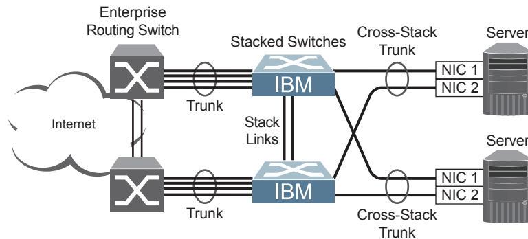
Figure 49. High Availability Topology Using Stacking
