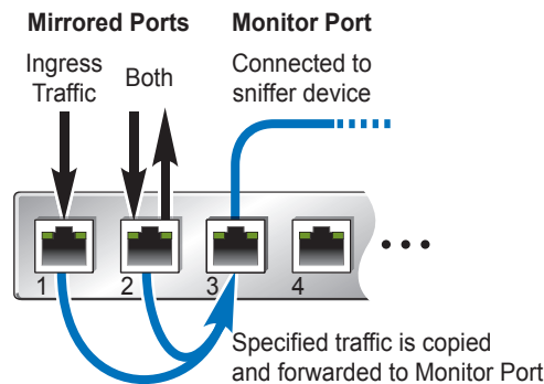
Figure 58. Mirroring Ports
