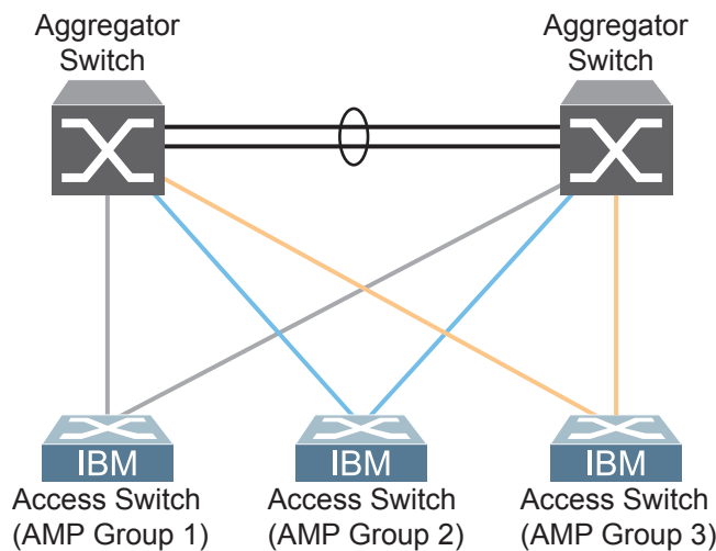
Figure 48. AMP Topology
