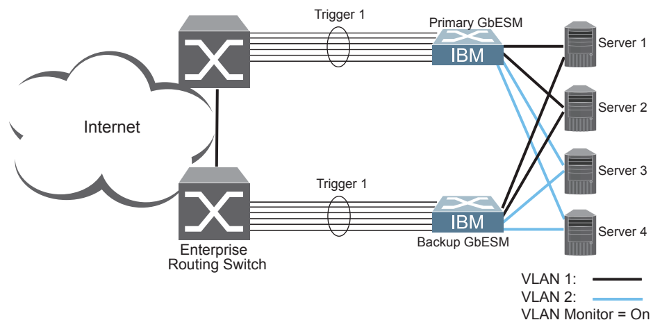
Figure 50. Basic Layer 2 Failover
