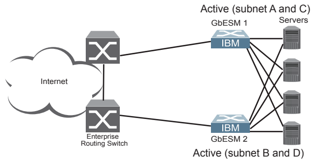
Figure 54. Active-Active Redundancy
