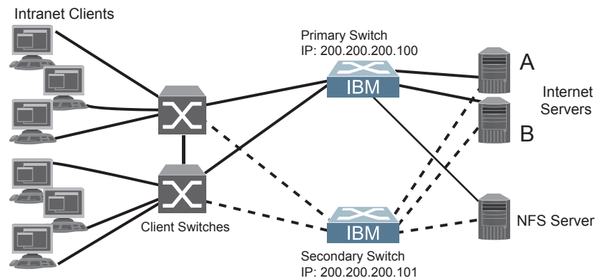
Figure 53 A Non-VRRP, Hot-Standby Configuration
