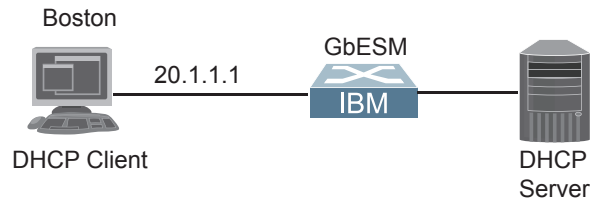
Figure 32. DHCP Relay Agent Configuration
