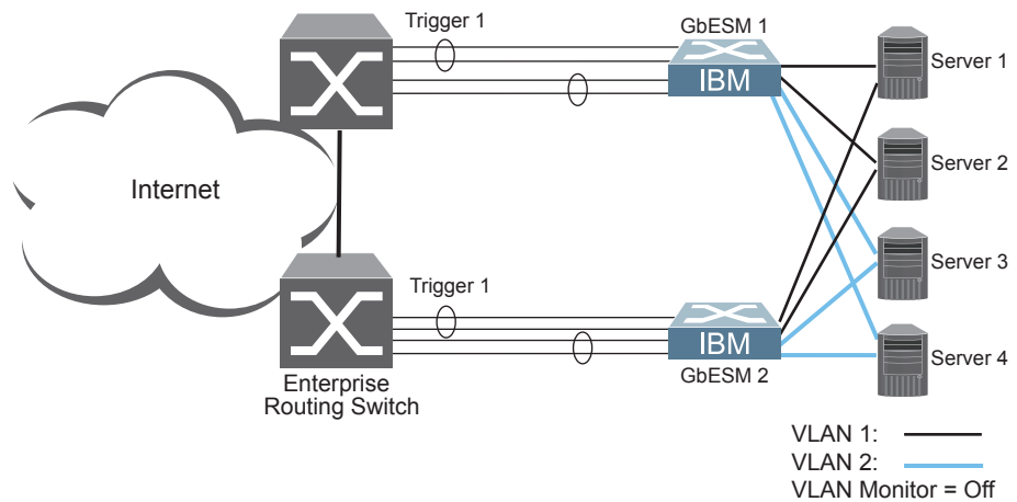
Figure 52. Two trunks, one Failover Trigger
