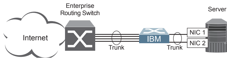
Figure 47. Trunking Ports for Link Redundancy
