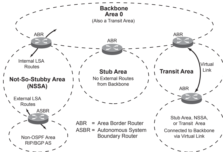
Figure 39. OSPF Area Types
