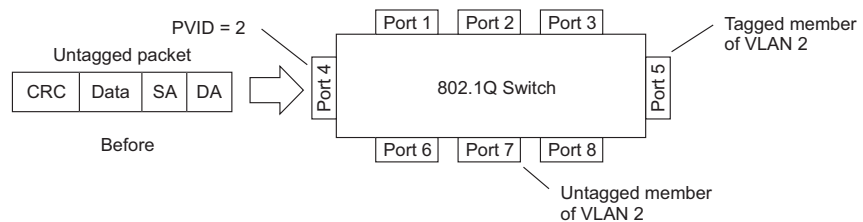
Figure 4. Port-based VLAN assignment
