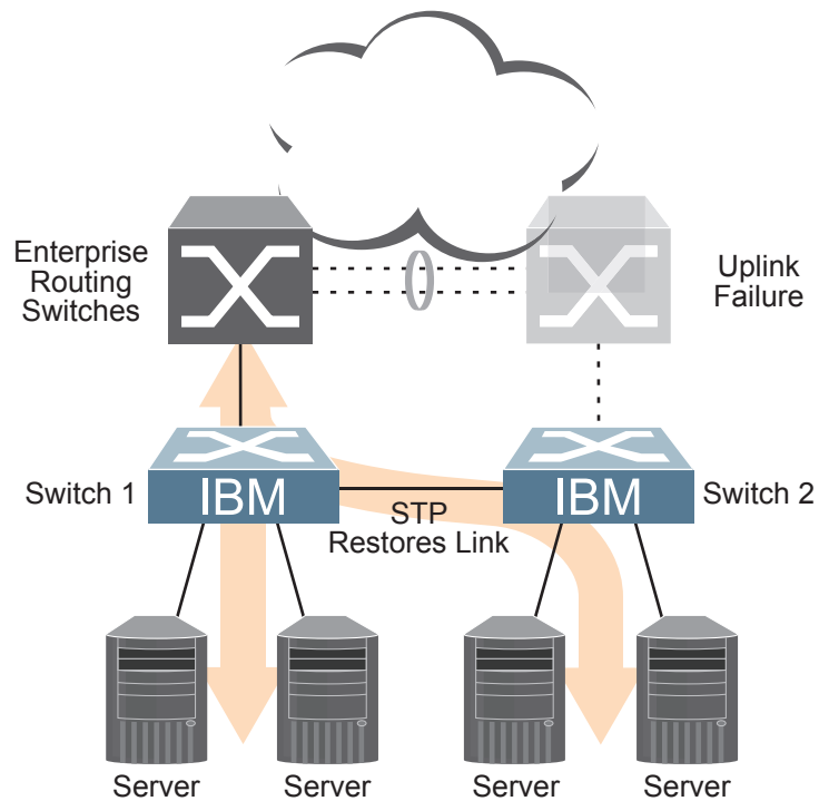
Figure 13. Spanning Tree Restoring the Switch-to-Switch Link
