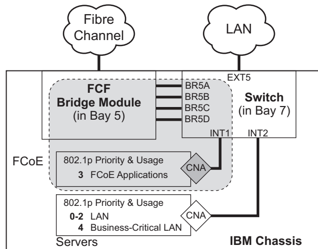
Figure 28. A Mixed Fibre Channel and FCoE Network
