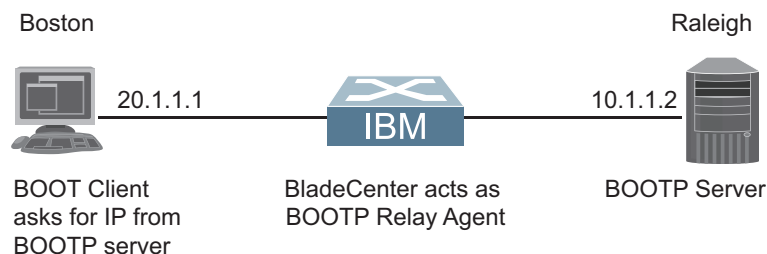
Figure 31. BOOTP Relay Agent Configuration
