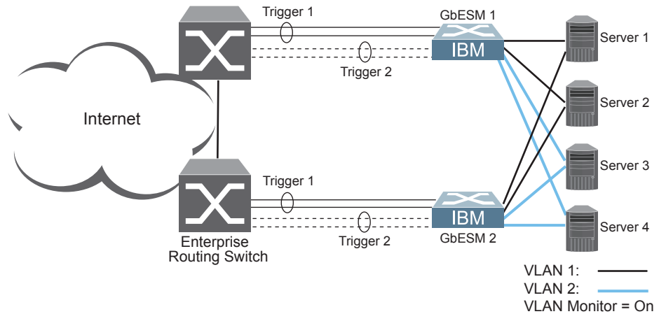
Figure 51. Two trunks, each in a different Failover Trigger
