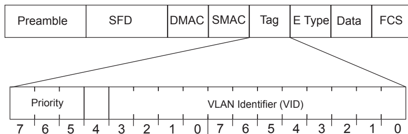
Figure 19. Layer 2 802.1q/802.1p VLAN Tagged Packet
