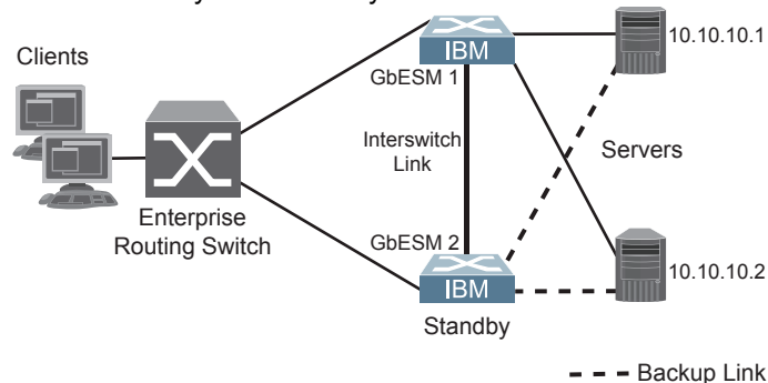
Figure 55. Hot-Standby Redundancy
