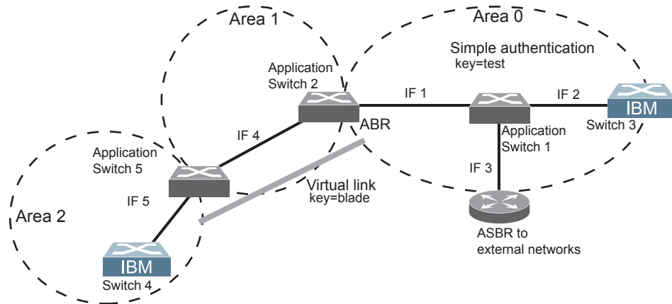
Figure 42. OSPF Authentication
