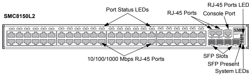
Figure 1-1 Front Panel
