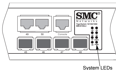
Figure 1-4 System LEDs
