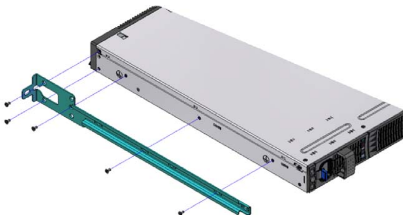
Figure 4: Screwing on the Rail
