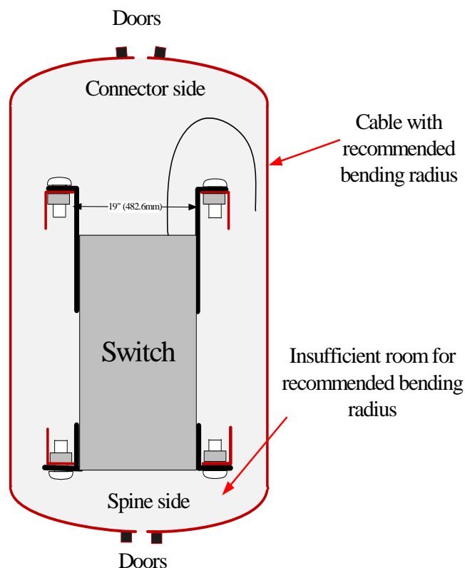
Figure 2: Placement of Switch in Rack
