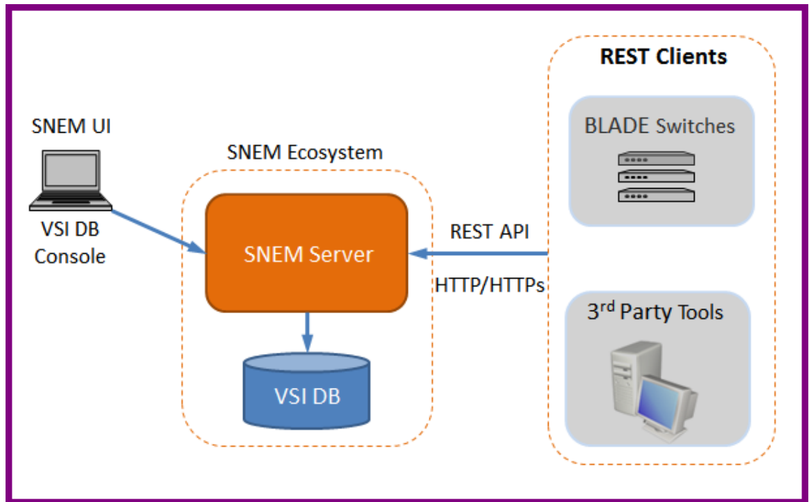
Figure 91 VSI database
