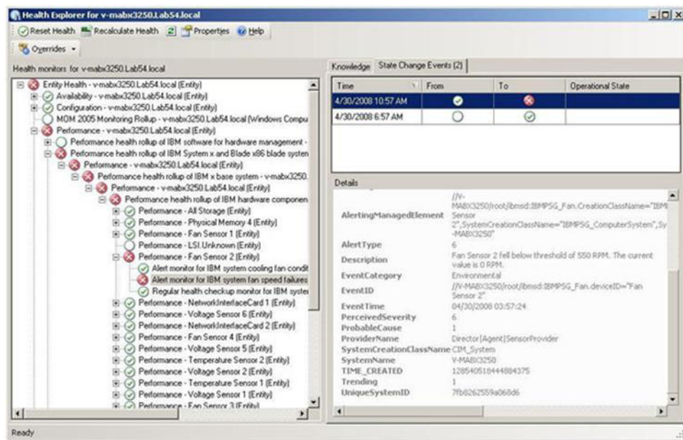
Figure 35. Example of hardware components causing a system to be in error
