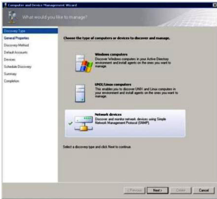
Figure 8. Discovery types
