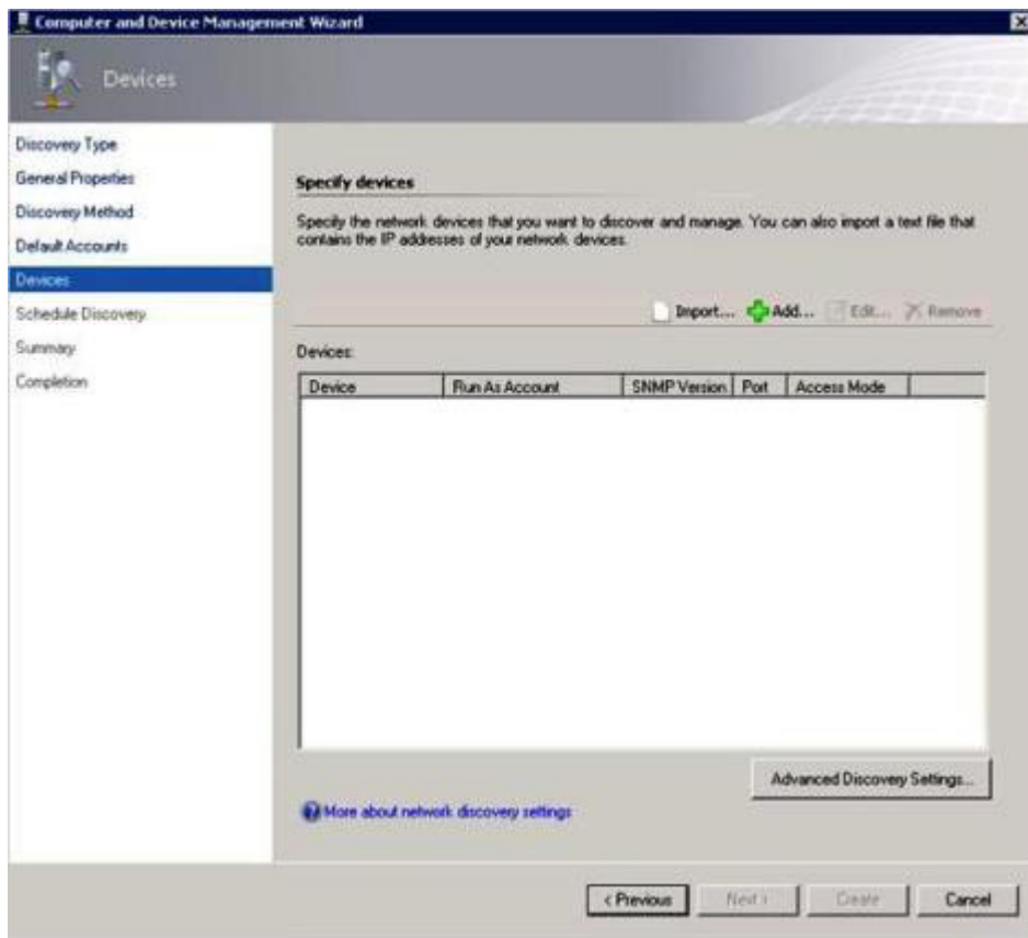
Figure 11. Devices page
