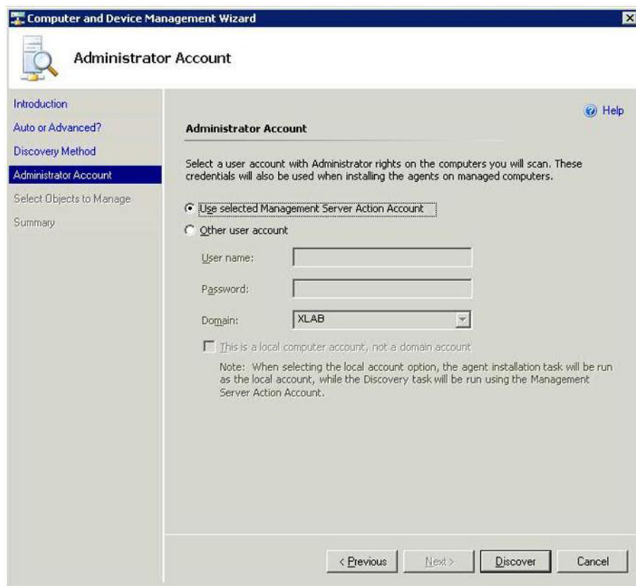
Figure 28. Administrator Account
