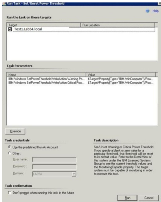
Figure 47. Target and task parameters of Set/Unset Power Threshold task
