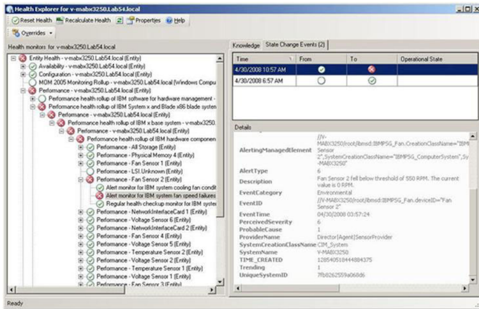
Figure 36. Example of a knowledge page that describes an error event
