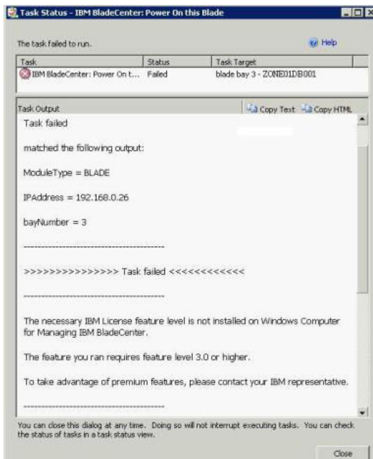
Figure 42. Example of a Task Output message
