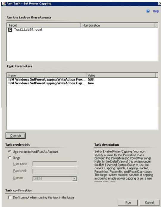
Figure 54. New values of the Task Parameters of Set Power Capping task
