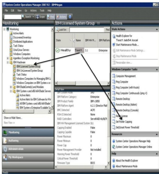
Figure 51. Example of Set Power Capping task
