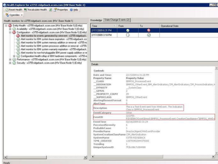
Figure 59. Example of the State Change Events tab detail information
