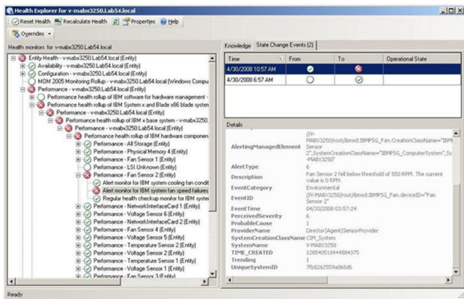
Figure 34. Example of hardware components causing a system to be in error
