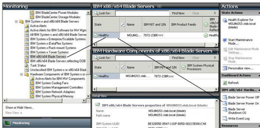
Figure 43. Example of Blade Server Power On task
