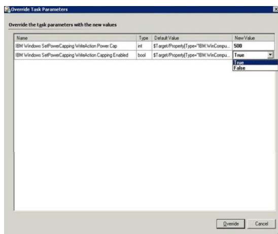
Figure 53. Override the Task Parameters of Set Power Capping task
