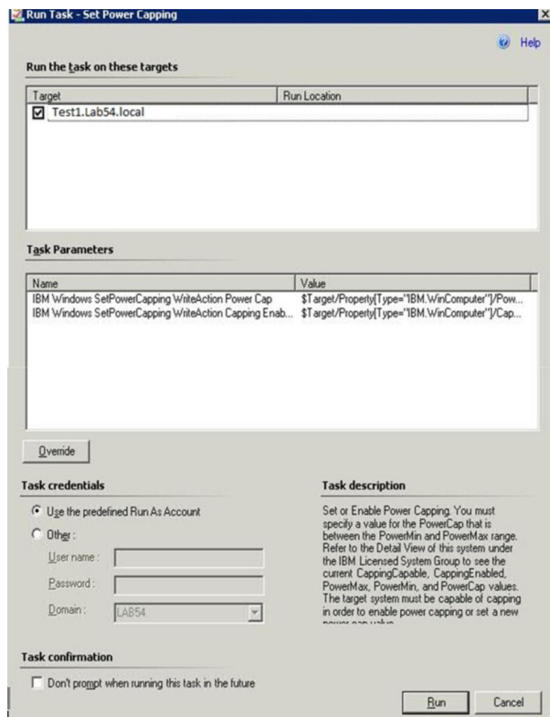
Figure 52. Target and task parameters of the Set Power Capping task
