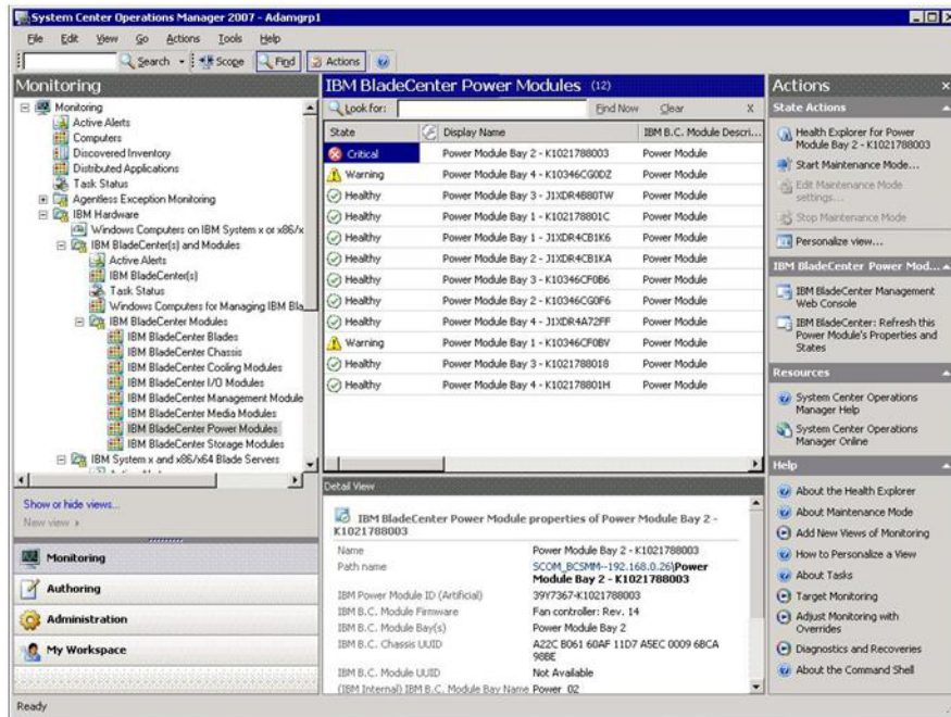
Figure 57. Detailed view of a power module in critical state
