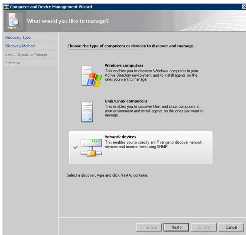
Figure 5. Discovery Wizard
