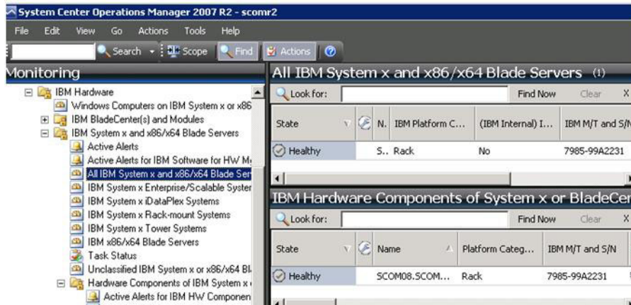
Figure 19. Dashboard view
