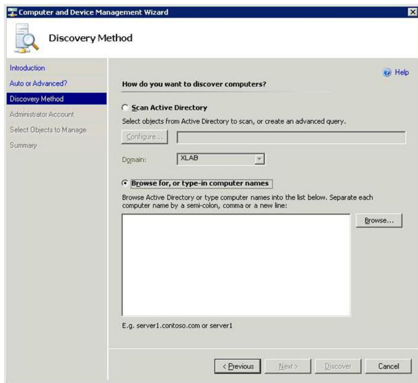
Figure 26. Discovery Method
