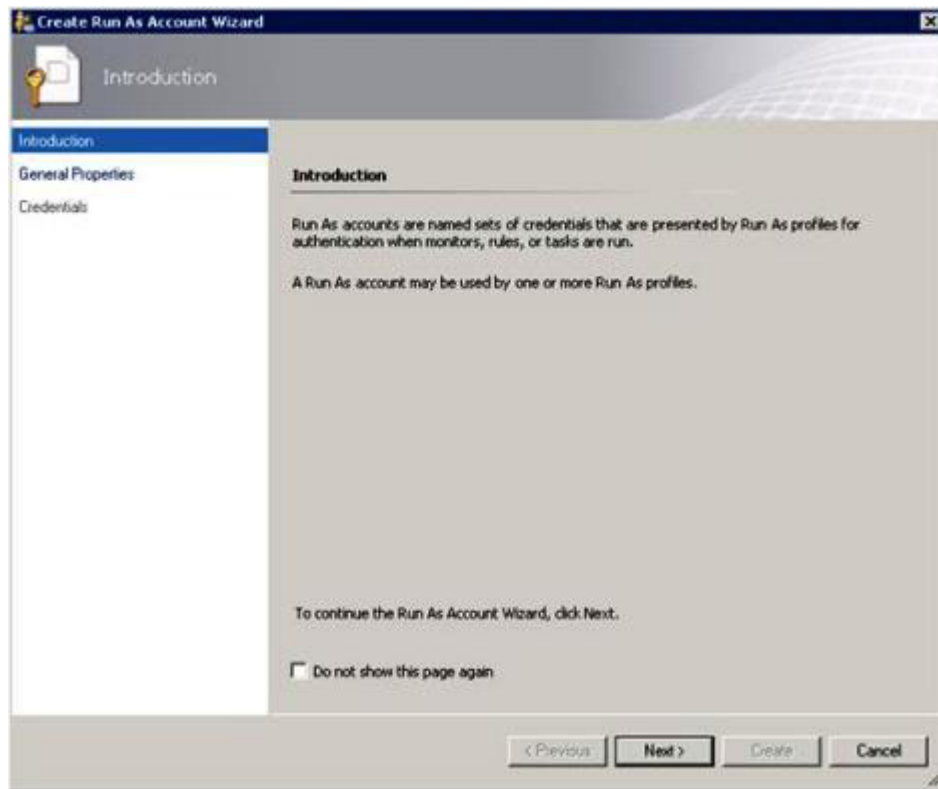
Figure 10. Introduction page
