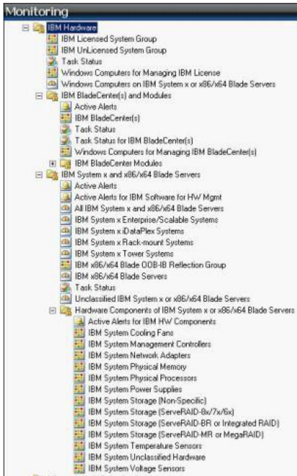
Figure 15. Monitoring pane
