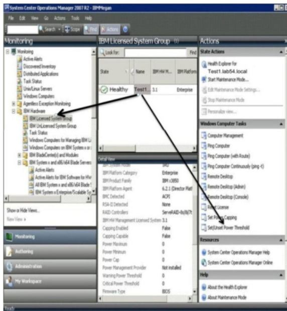
Figure 46. Example of Set/Unset Power Threshold task
