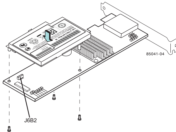
Figure 5.2 Installing the iBBU Daughtercard on the ServerRAID M5025 SAS/SATA Controller
