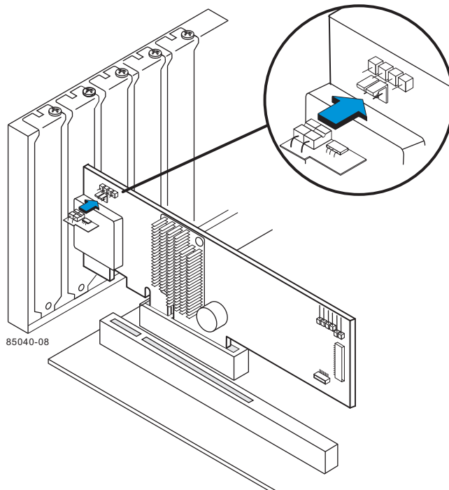
Figure 8.2 Installing the ServeRAID M5000 Series Advanced Feature Key on the M5025 ServeRAID SAS/SATA Controller
