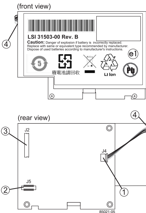
Figure 5.1 Intelligent Battery Backup Unit
