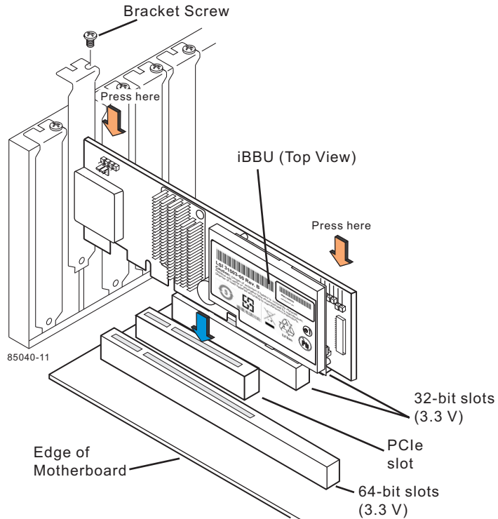
Figure 2.1 ServerRAID M5025 Controller Installation in a PCI Express Slot
