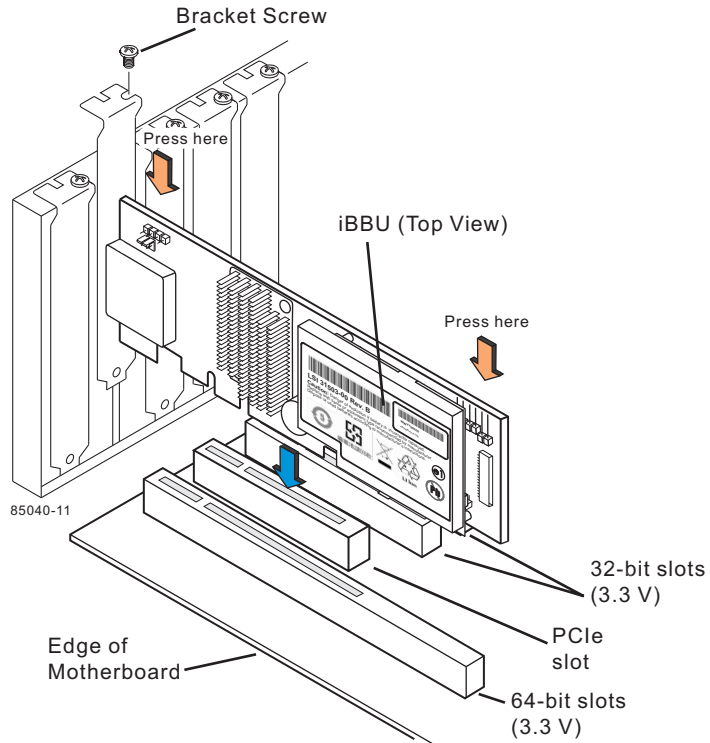
Figure 5.3 Installing the ServeRAID M5025 SAS/SATA Controller
