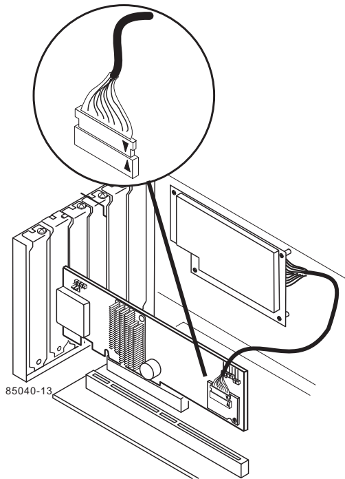
Figure 5.4 Connecting the iBBU Remotely to the ServeRAID M5025 SAS/SATA Controller
