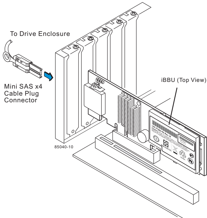
Figure 2.2 Connecting the ServeRAID M5025 Controller to a Drive Enclosure
