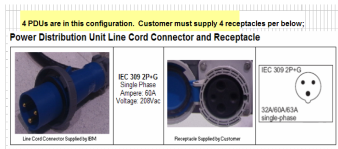
Figure 2: Example of IBM BladeCenter Foundation for Cloud on System x US Cord Connectors
