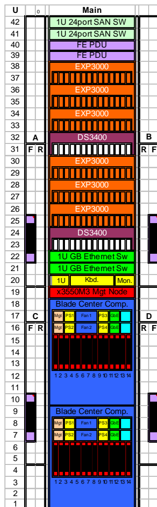
Figure 1: Example of Large IBM BladeCenter Foundation for Cloud on System x Rack
