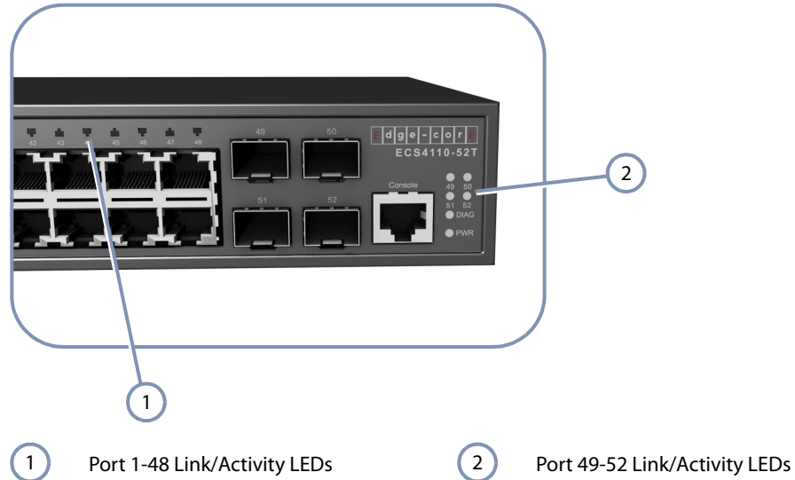
Figure 15: Port Status LEDs
