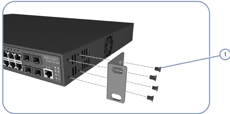
Figure 8: Attaching the Brackets
