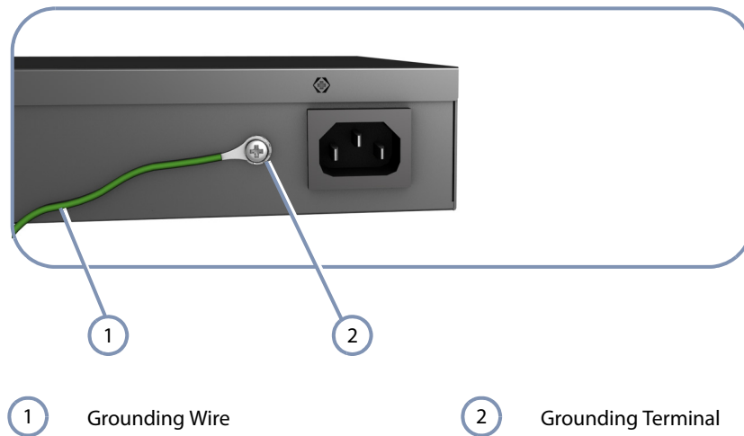
Figure 13: Grounding Terminal
