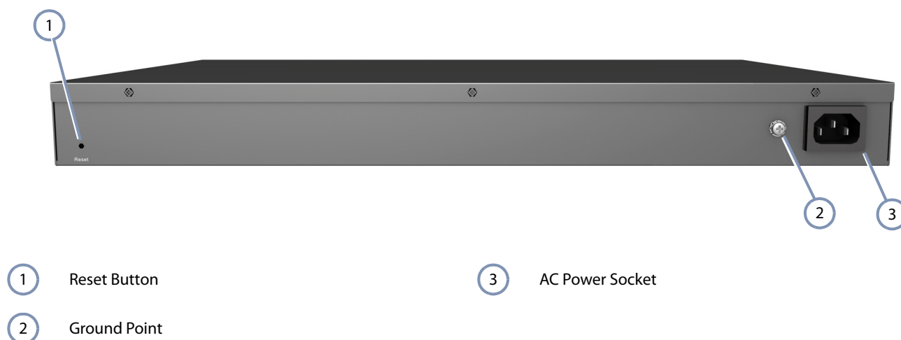
Figure 2: Rear Panel
