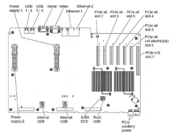
Figure 1. System x3850 X5 I/O-board connectors
