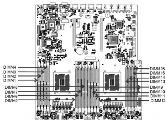
Figure 1. System Board DIMM Connectors
