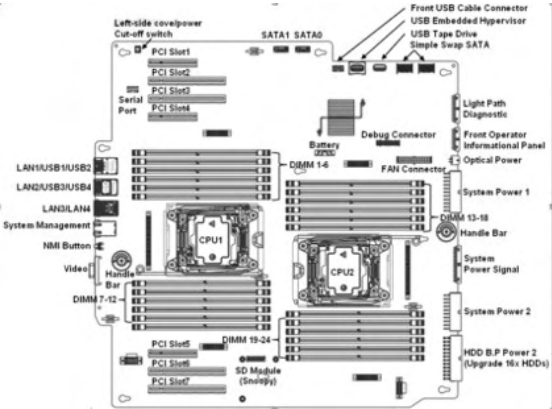
Figure 1. x3500 M5 Slots
