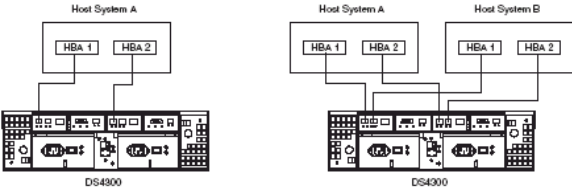
Figure 3. DS4100 and DS4300 Drive Attach Examples
