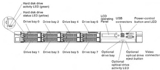
Figure 2. 2.5" Model Front View (10x 2.5")
