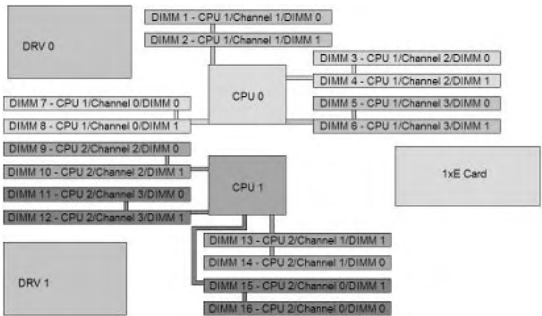
Figure 1. Memory logical connections
