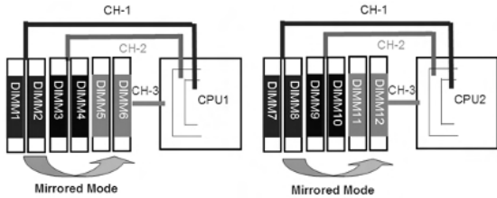
Figure 2. Memory channel interface layout for mirrored mode
