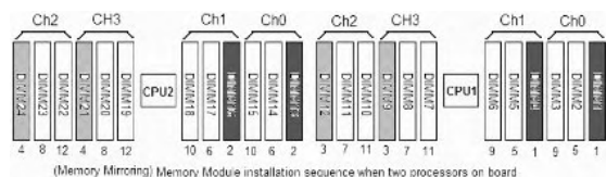
Figure 3. Memory Mirroring mode DIMM population rules
