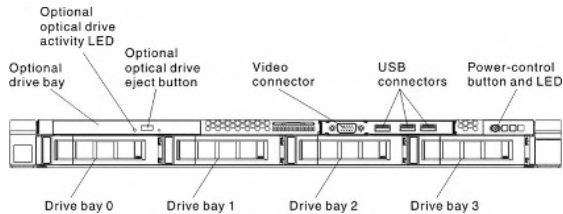
Figure 3. 3.5" Model Front View (4x 3.5")
