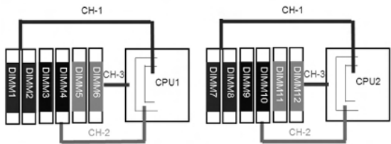
Figure 2. Memory channel interface layout for mirrored mode
