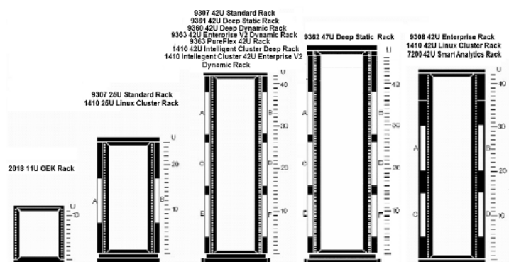
Figure 1. Rack cabinets
