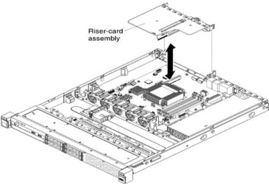
Figure 2. Riser Card Assembly
