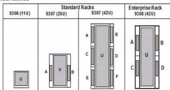
Figure 2. Side-wall Compartment Arrangements
