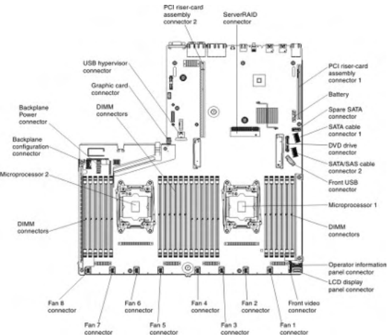
Figure 1. System planar
