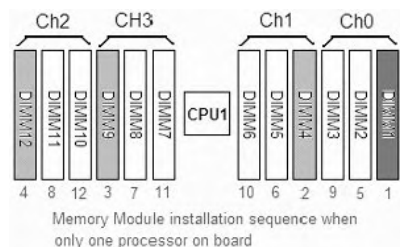
Figure 2. Memory DIMM assignment and installation sequence (two CPU)
