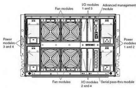
Figure 2. BladeCenter S (8886) rear view
