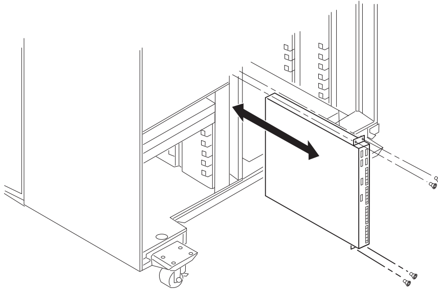
FIGURE 1 Insert the IBM Ethernet Switch B24X into a vertical mounting slot
