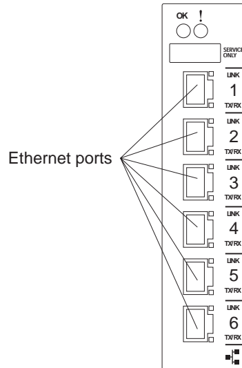
Figure 1 SCM faceplate
