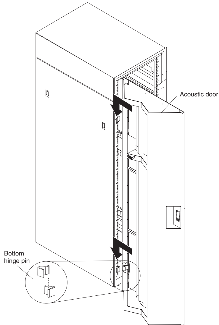
Figure 2. Installing an acoustic door on the rear of the rack cabinet
