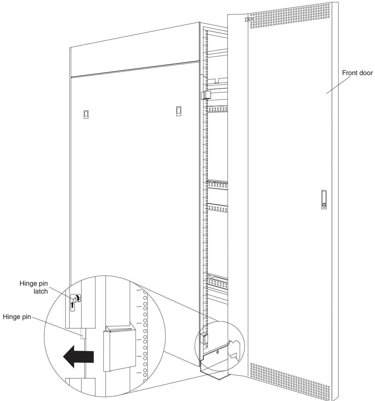
Figure 3. Removing the rack cabinet front door
