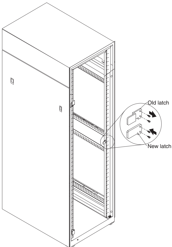
Figure 5. Removing and installing the front door latch plate
