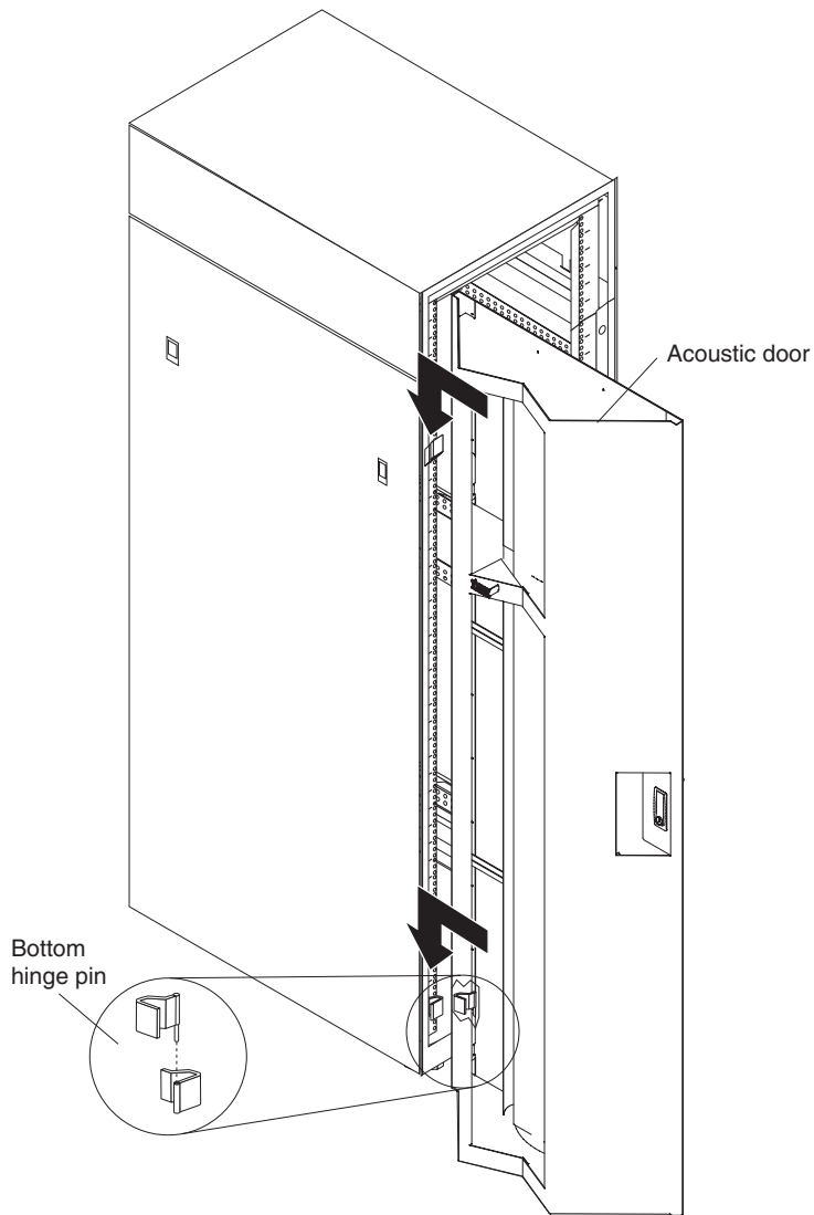
Figure 6. Installing an acoustic door on the front of the rack cabinet
