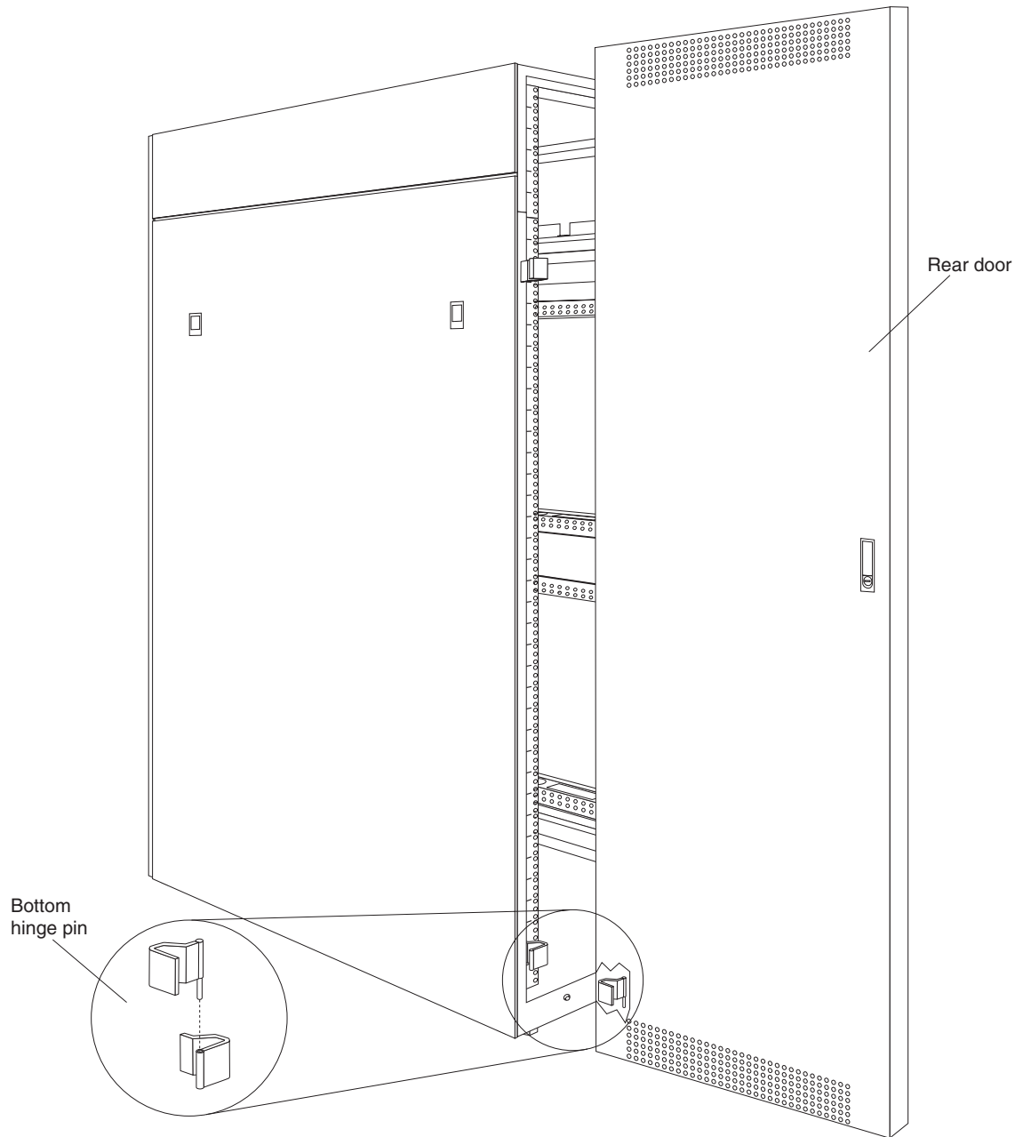
Figure 1. Removing the rack cabinet rear door
