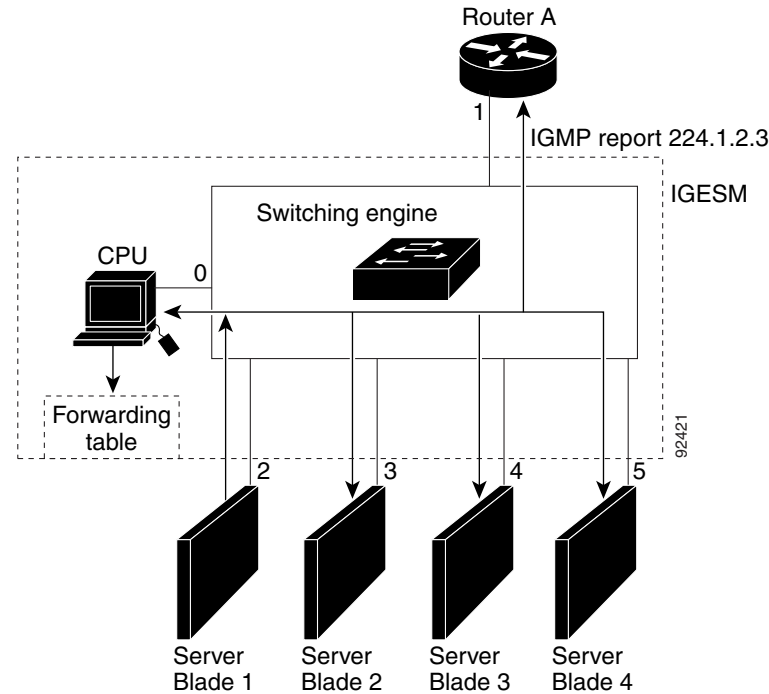
Figure 14-1 Initial IGMP Join Message
