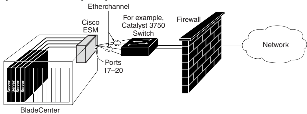
Figure 1-2 Trunking Configuration
