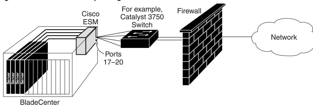
Figure 1-3 Redundancy Configuration
