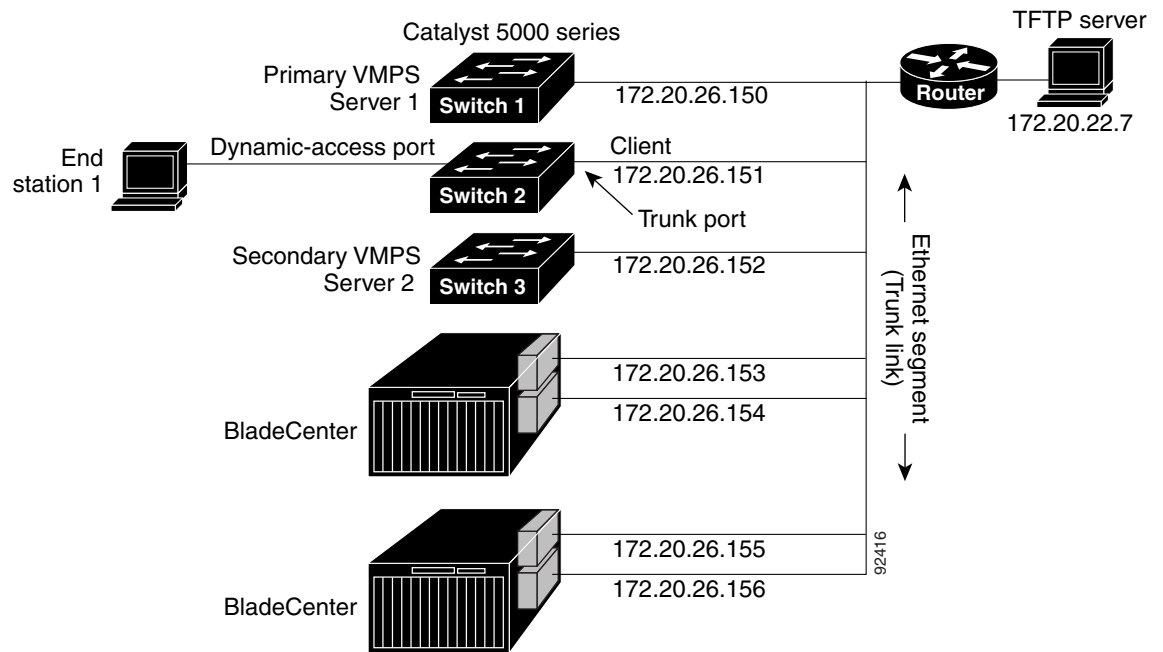
Figure 12-5 Dynamic Port VLAN Membership Configuration
