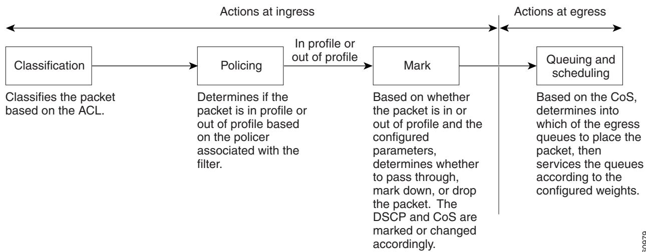
Figure 23-2 Basic QoS Model
