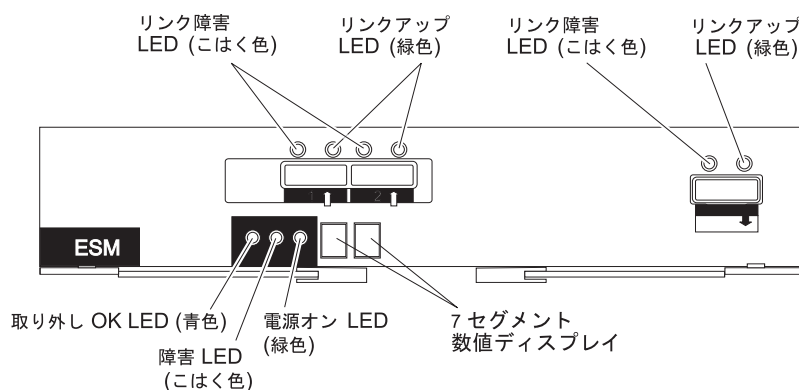
図 58. ESM LED
