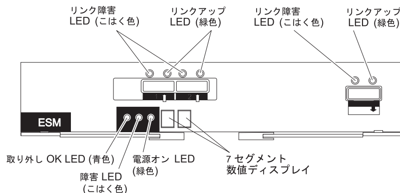
図 55. ESM LED
