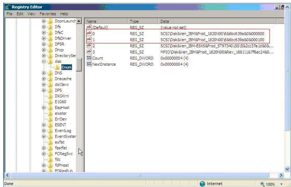
Figure 57. An example of \HKEY_LOCAL_MACHINE\SYSTEM\CurrentControlSet\Services\disk\Enum key
