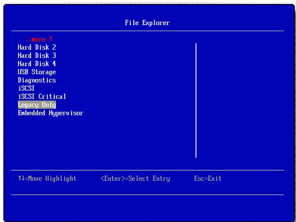
Figure 155. Legacy only
