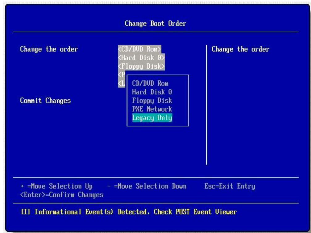
Figure 156. Legacy only
