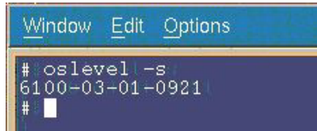
Figure 112. oslevel -s
