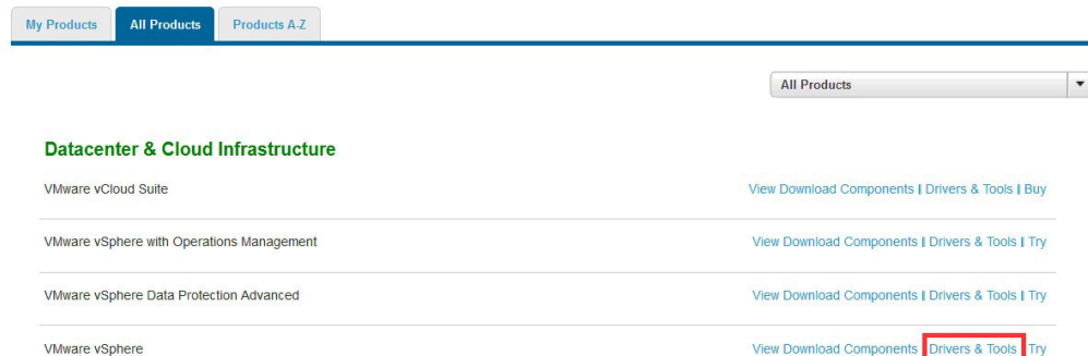
Figure 80. Drives & Tools
