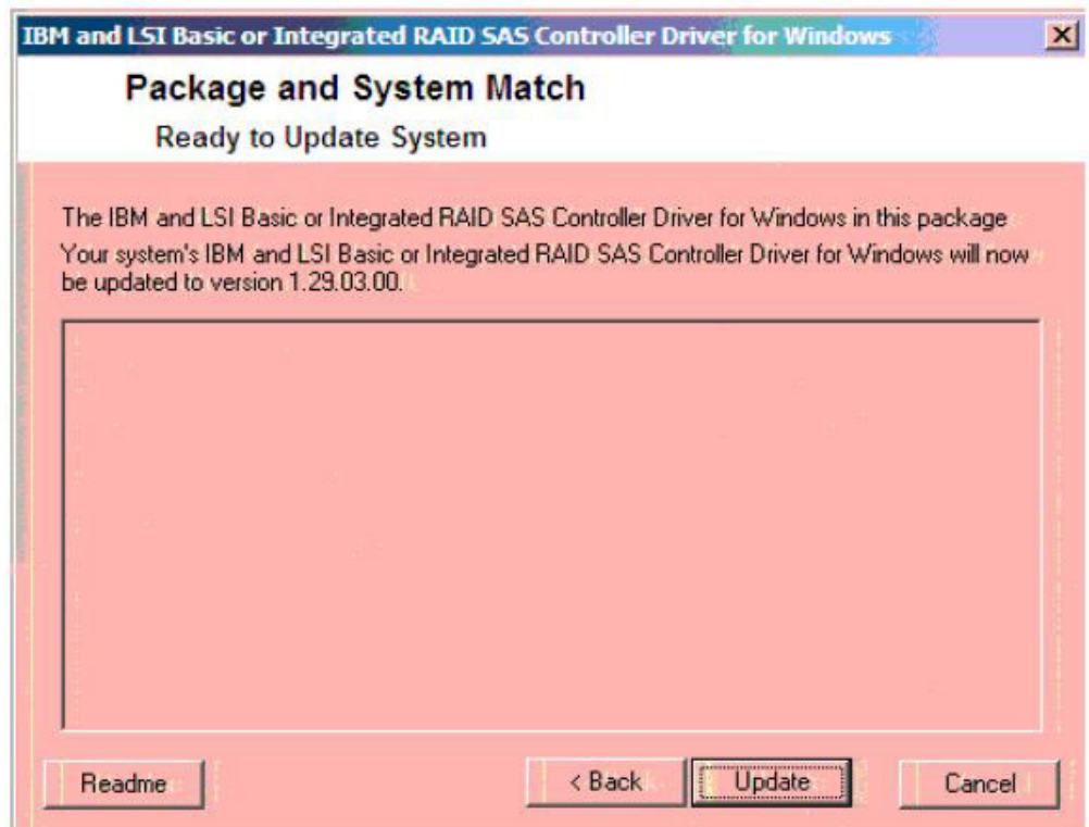
Figure 45. Click Update
