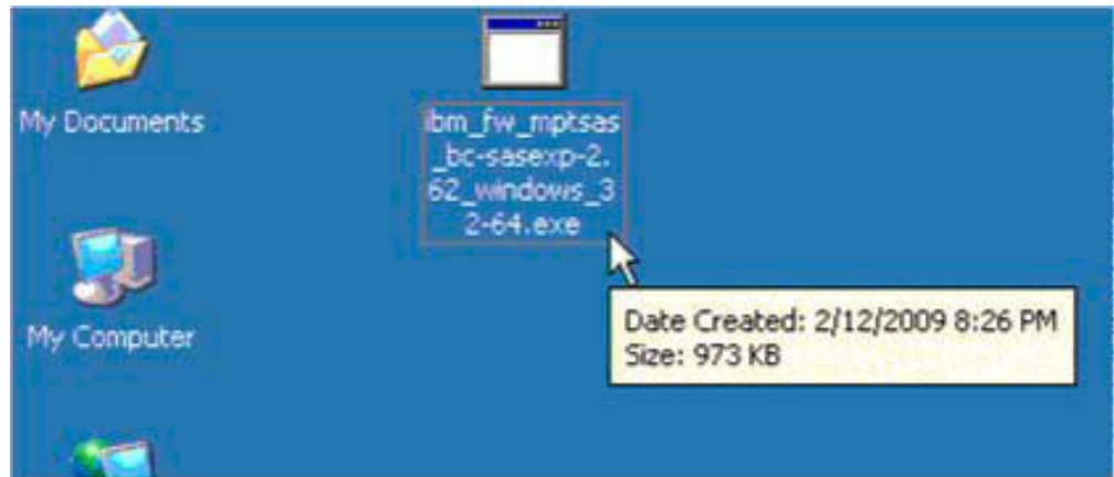
Figure 51. ibm_fw_mptsas_bc-sasexp-2.62_windows_32-64.exe
