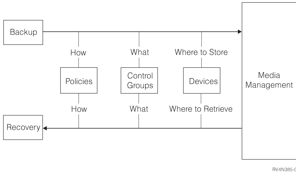
(artname: RV4N385.EPS) Figure 2. How the standard functions work together
