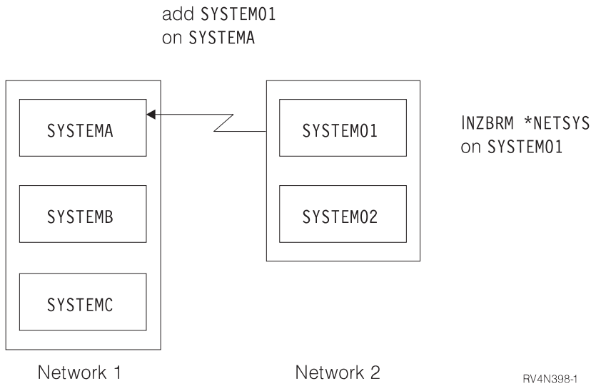
Figure 13. The wrong way to join two BRMS networks
