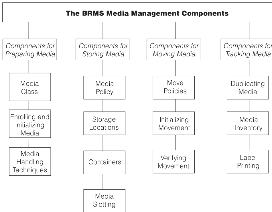
(artname: RV4N387.EPS) Figure 6. The BRMS Media Management Components
