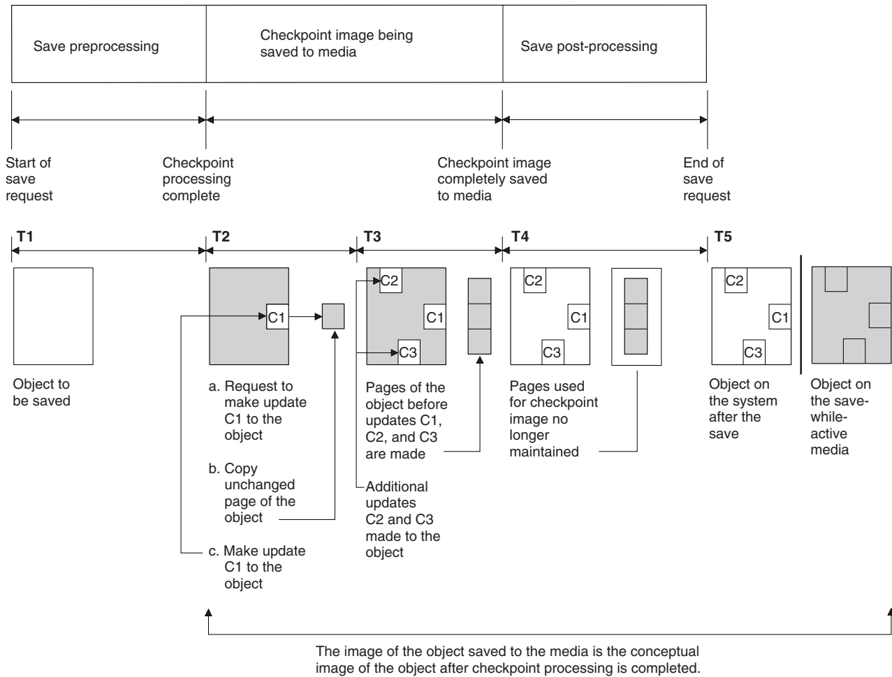
Figure 6. System management of updates to objects after checkpoint processing is complete
