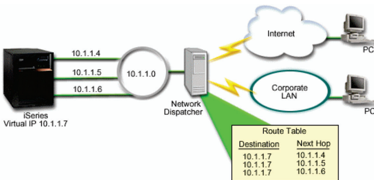
Figure 1. Adapter failover without local clients
