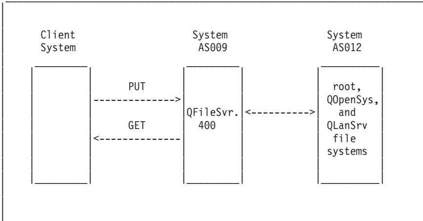
Figure 9-31. Subcommands to Transfer Files Using QFileSvr.400
