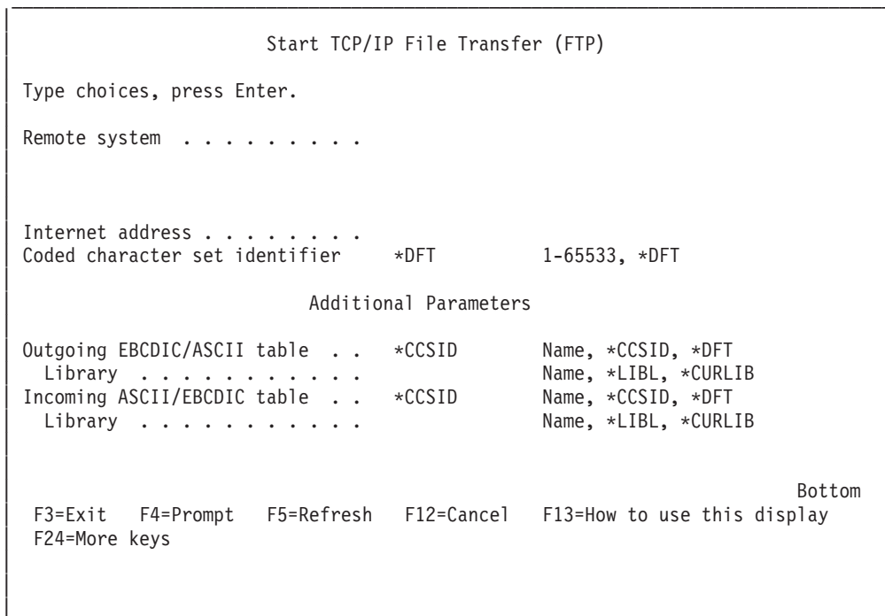
Figure 1. Specifying ASCII Mapping Tables with the *CCSID Value
