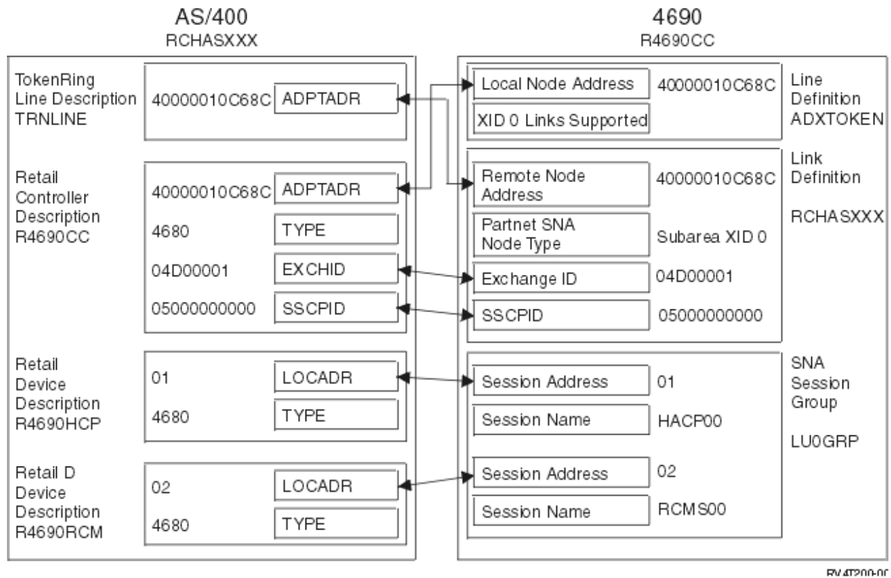
Example 2: iSeries server to 4690 PEER connection over token-ring network
