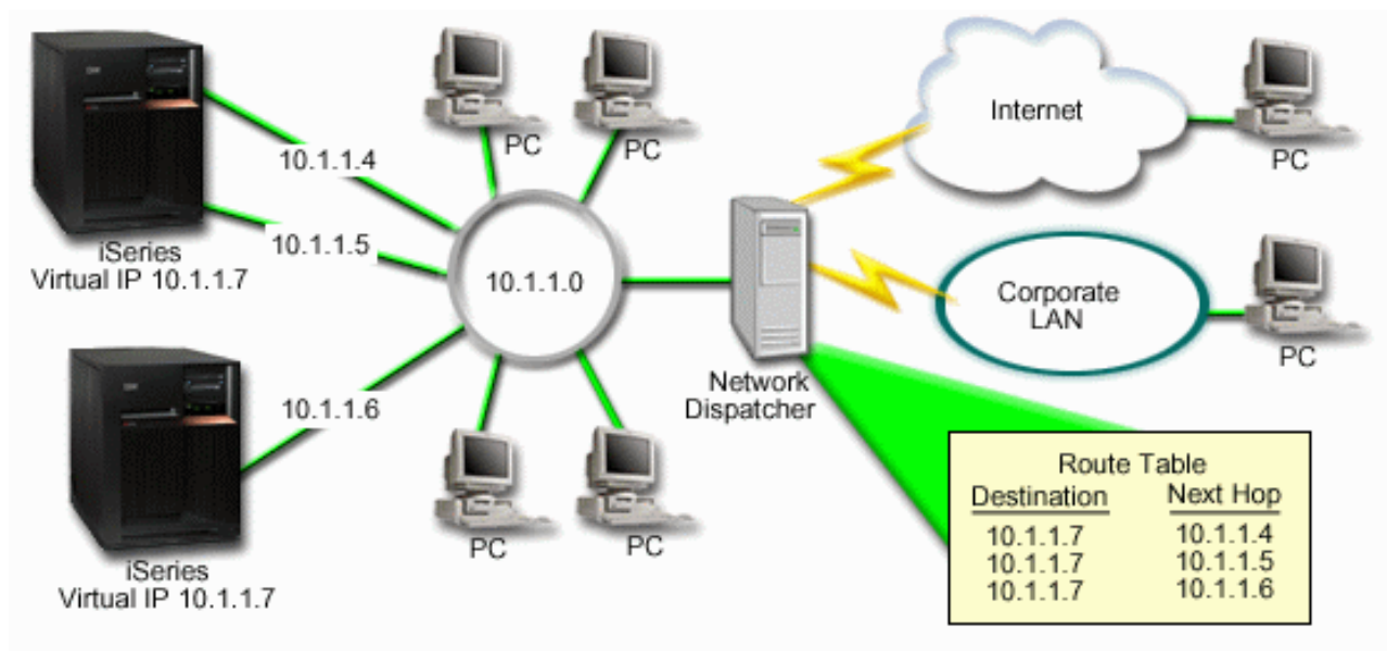
Figure 2. Adapter failover with local clients
