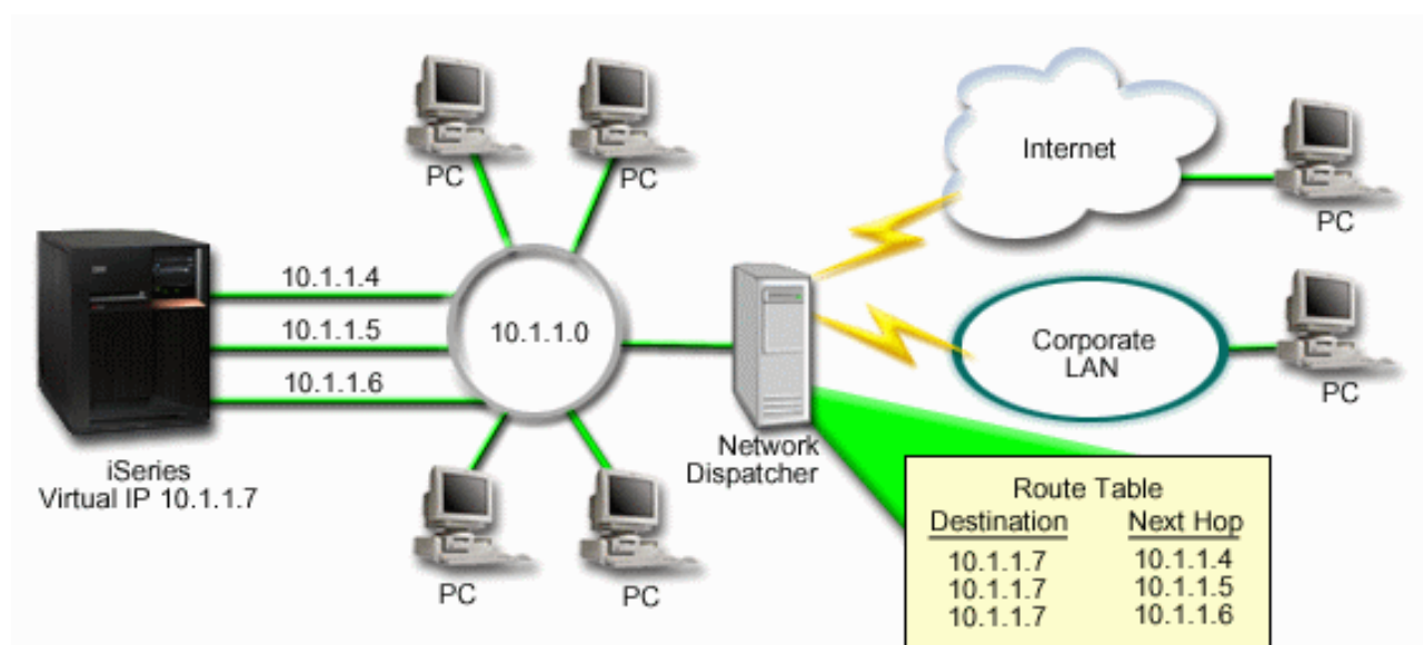
Figure 1. Adapter failover without local clients
