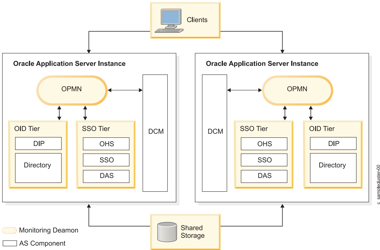
Figure 1. Basic Oracle Application Server for CFC configuration
