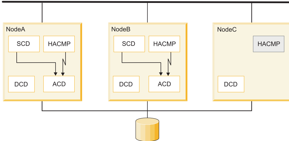
Synchronization 3: Dynamic reconfiguration complete; cluster services started on NodeC
