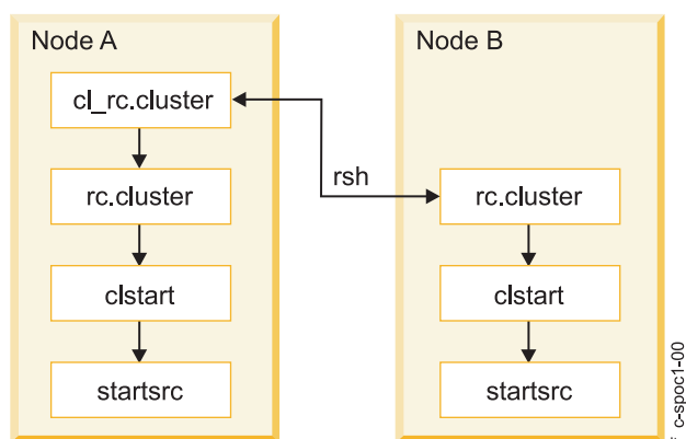
Figure 30. Flow of commands used at cluster startup by C-SPOC utility
