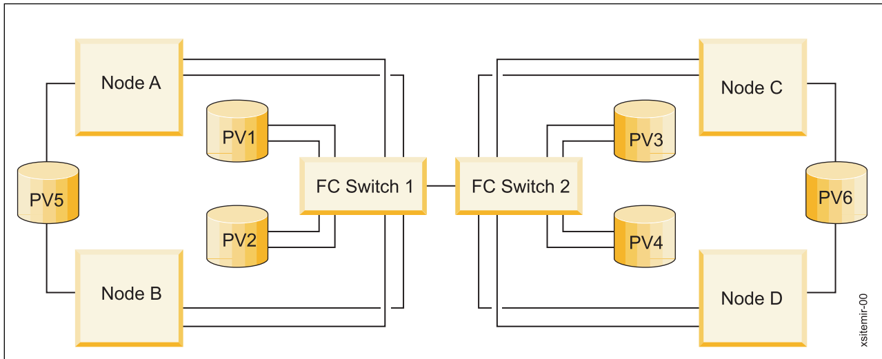
Figure 28. Cross-site LVM mirroring configuration with a SAN
