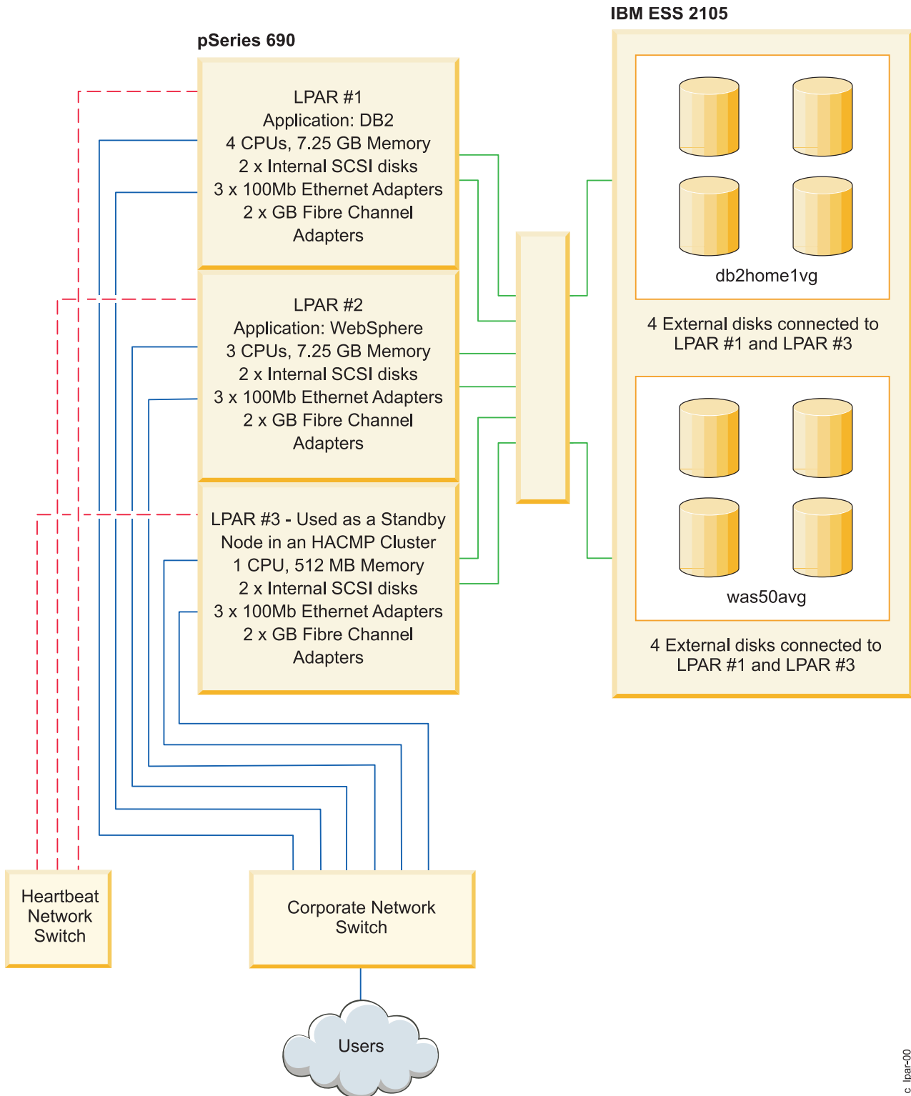
Figure 29. Cluster with three LPARs
