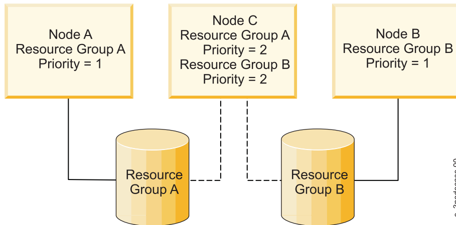
Figure 20. One-for-two standby configuration with three resource groups
