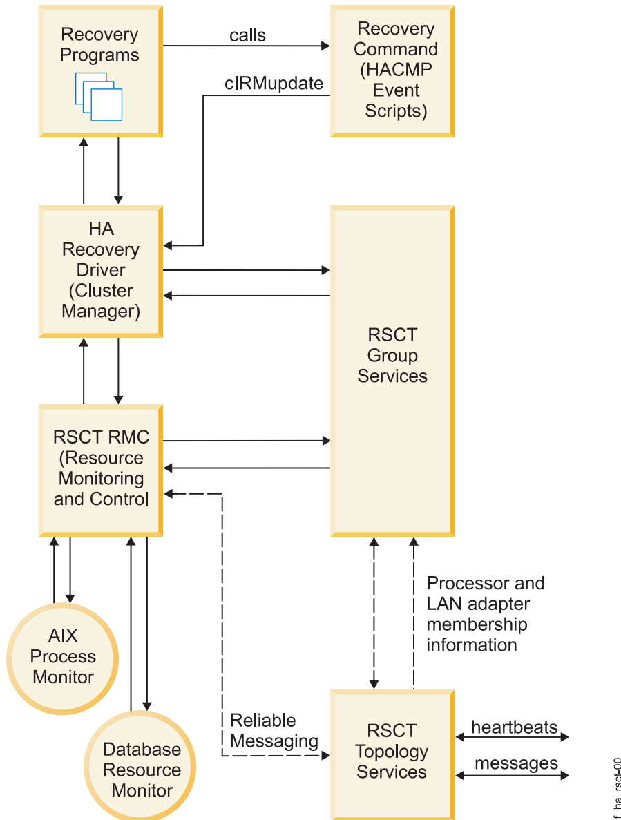
Figure 8. Components of PowerHA SystemMirror architecture
