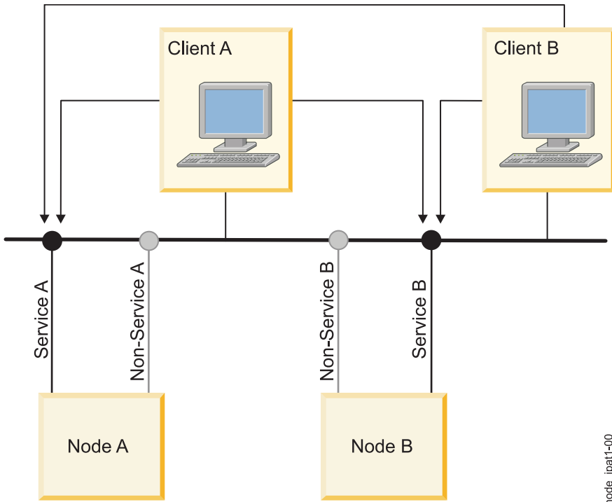
Figure 9. Concurrent access configuration before disk takeover
