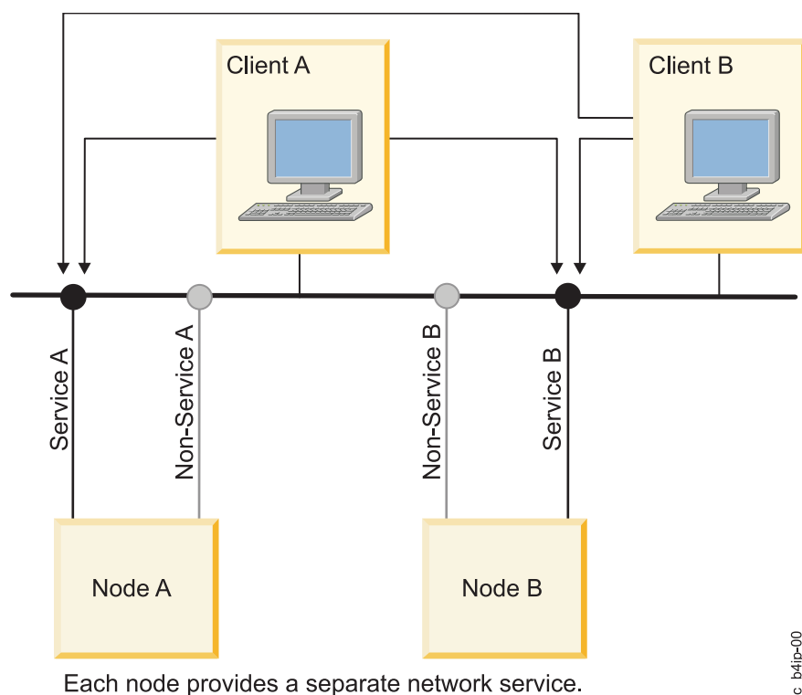
Figure 11. Configuration before IP address takeover via IP replacement
