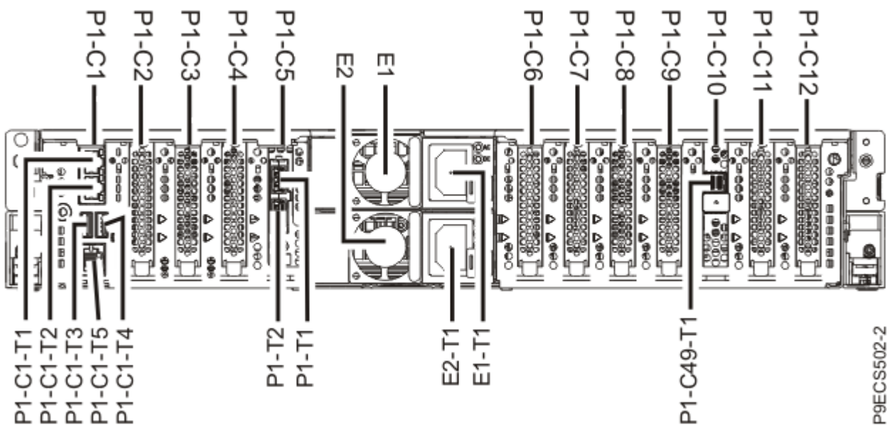
Figure 1. Rear view of a rack-mounted 5105-22E, 9009-22G, or 9223-22S system with PCIe4 slots location codes
