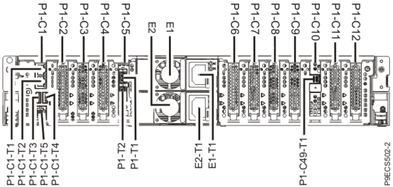
Figure 2. Rear view of a rack-mounted 9008-22L, 9009-22A, or 9223-22H system with PCIe slots location codes
