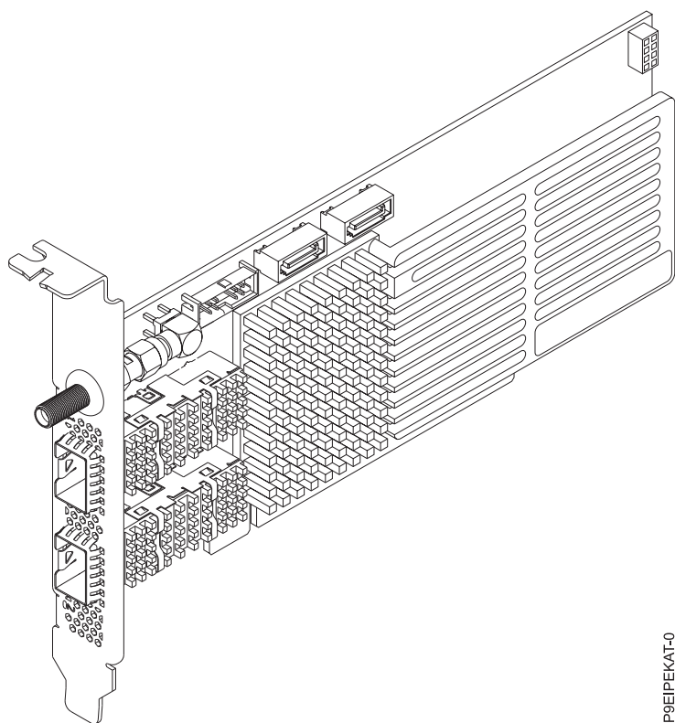
Figura 38. AlphaData ADM-PCIE-9V3 CAPI2.0 FPGA (Xilinx VU3P) Dev Kit PCIe4 x8
