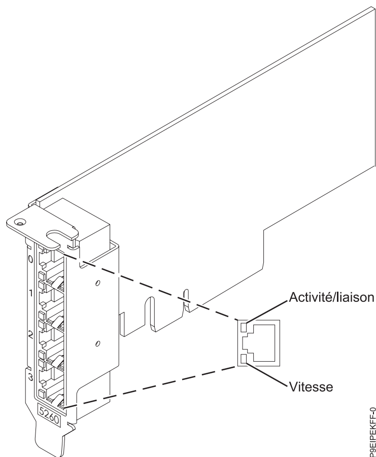
Figure 47. Broadcom 5719 QP 1G (1G/100M/10M) Network Interface Card PCIe x4 LP
