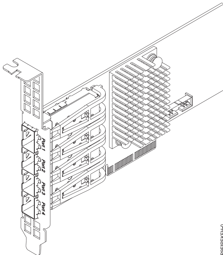
Figure 48. Carte Intel XL710 Ethernet Converged Network Adapter quatre ports 10G/1G SFP+ PCIe3.0 x8 LP
