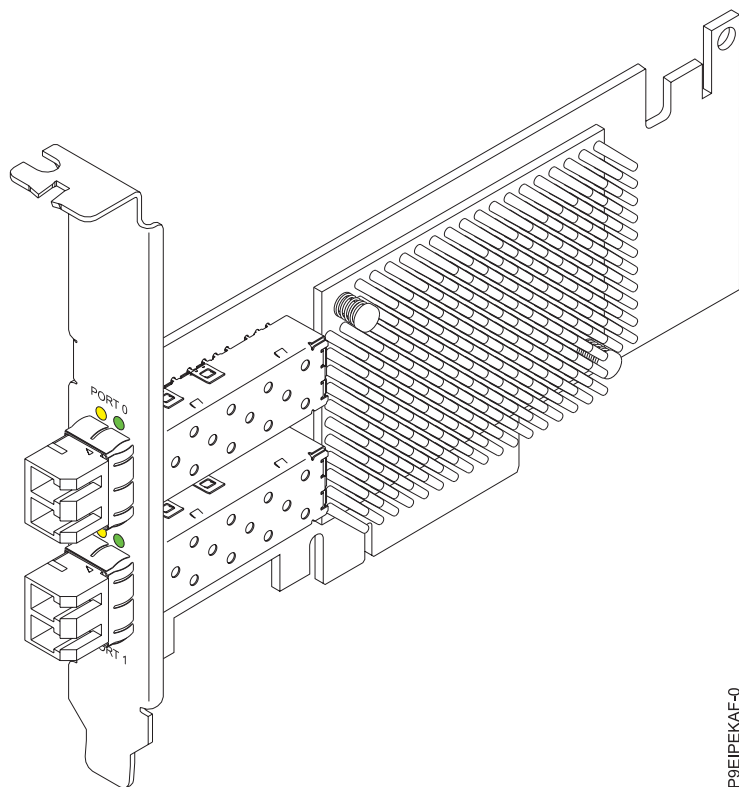
Figure 31. Carte Fibre Channel Emulex LPE16002B-M6-O double port 16 Go PCIe3.0 x8 LP
