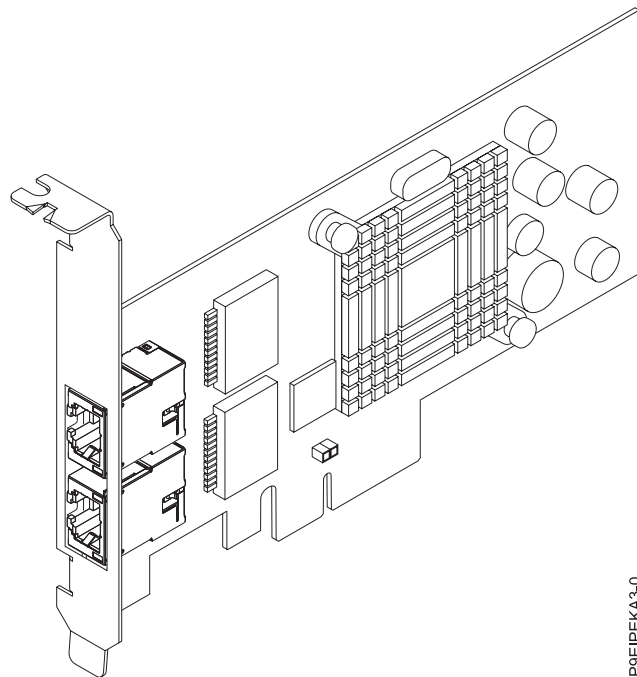
Figure 28. ICarte Intel 82575EB double port Gigabit Ethernet Controller PCIe x4.0 LP
