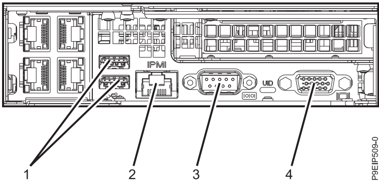
Figure 2. Ports arrière
