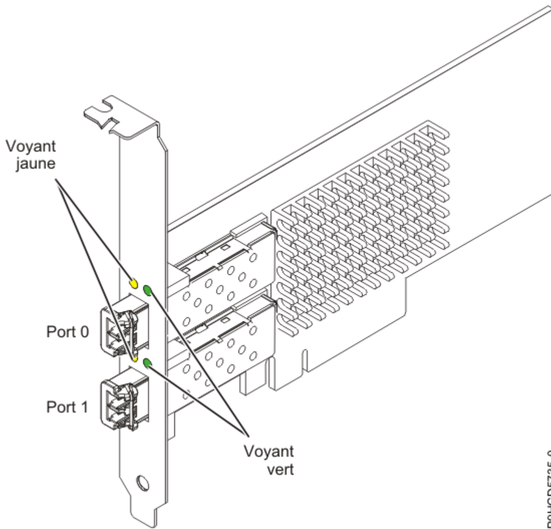
Figure 25. Carte PCIe3 LP 16 Gb 2 ports Fibre Channel
