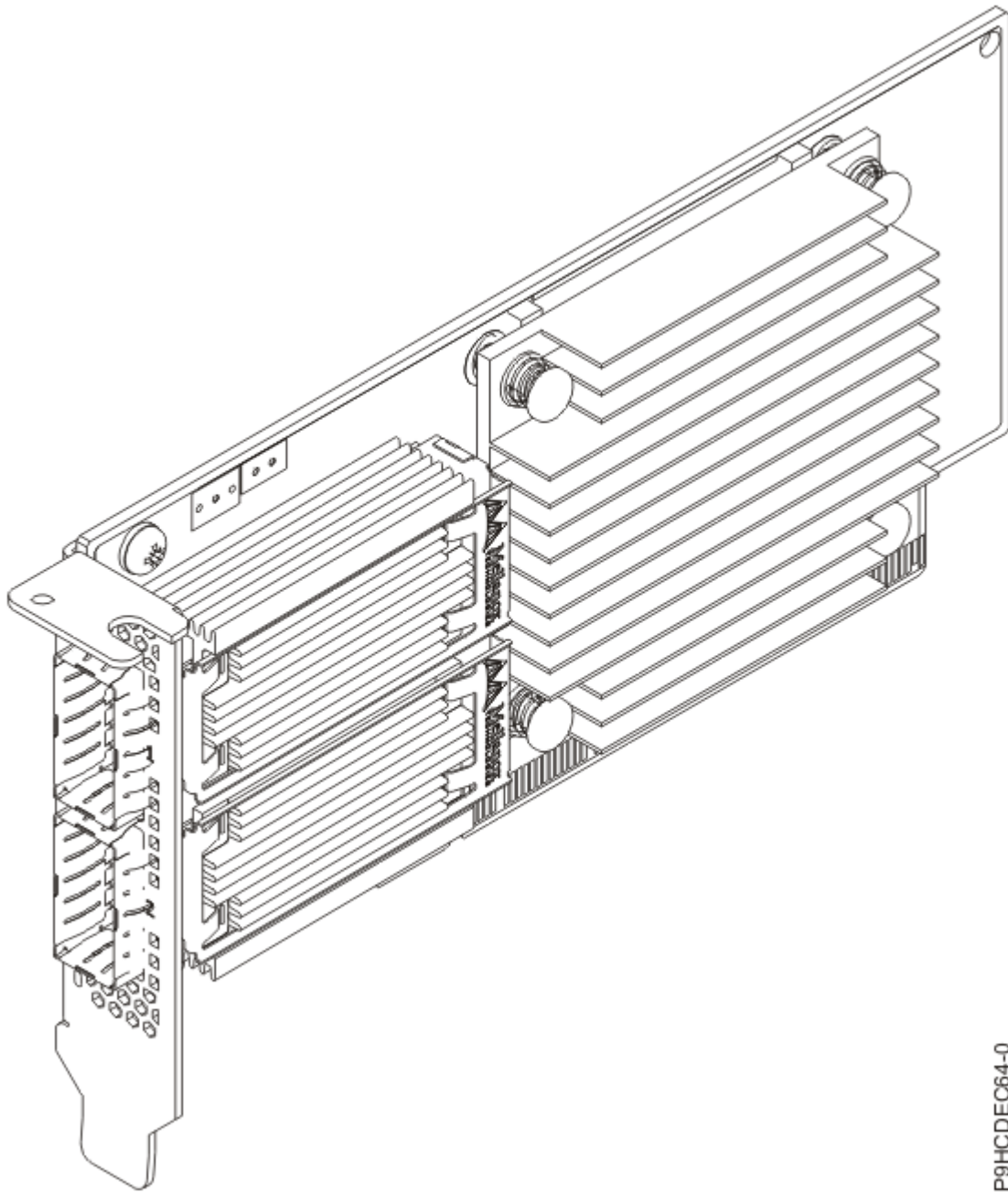
Figure 22. Carte PCIe4 x16 2 ports EDR 100 GB IB ConnectX-5 compatible CAPI
