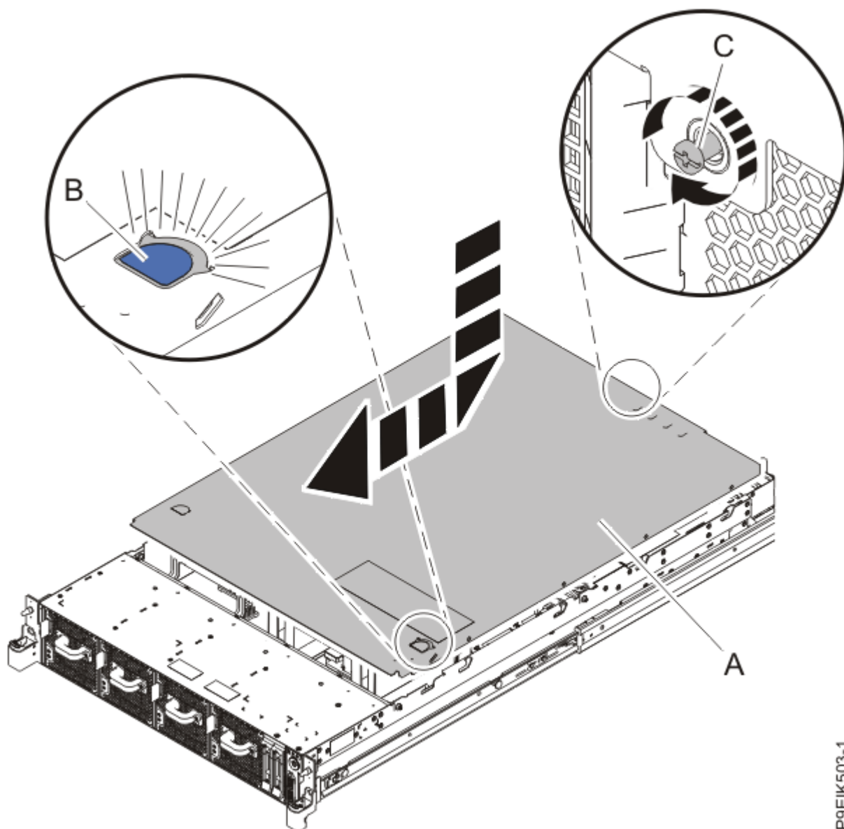
Figure 42. Installation du capot
