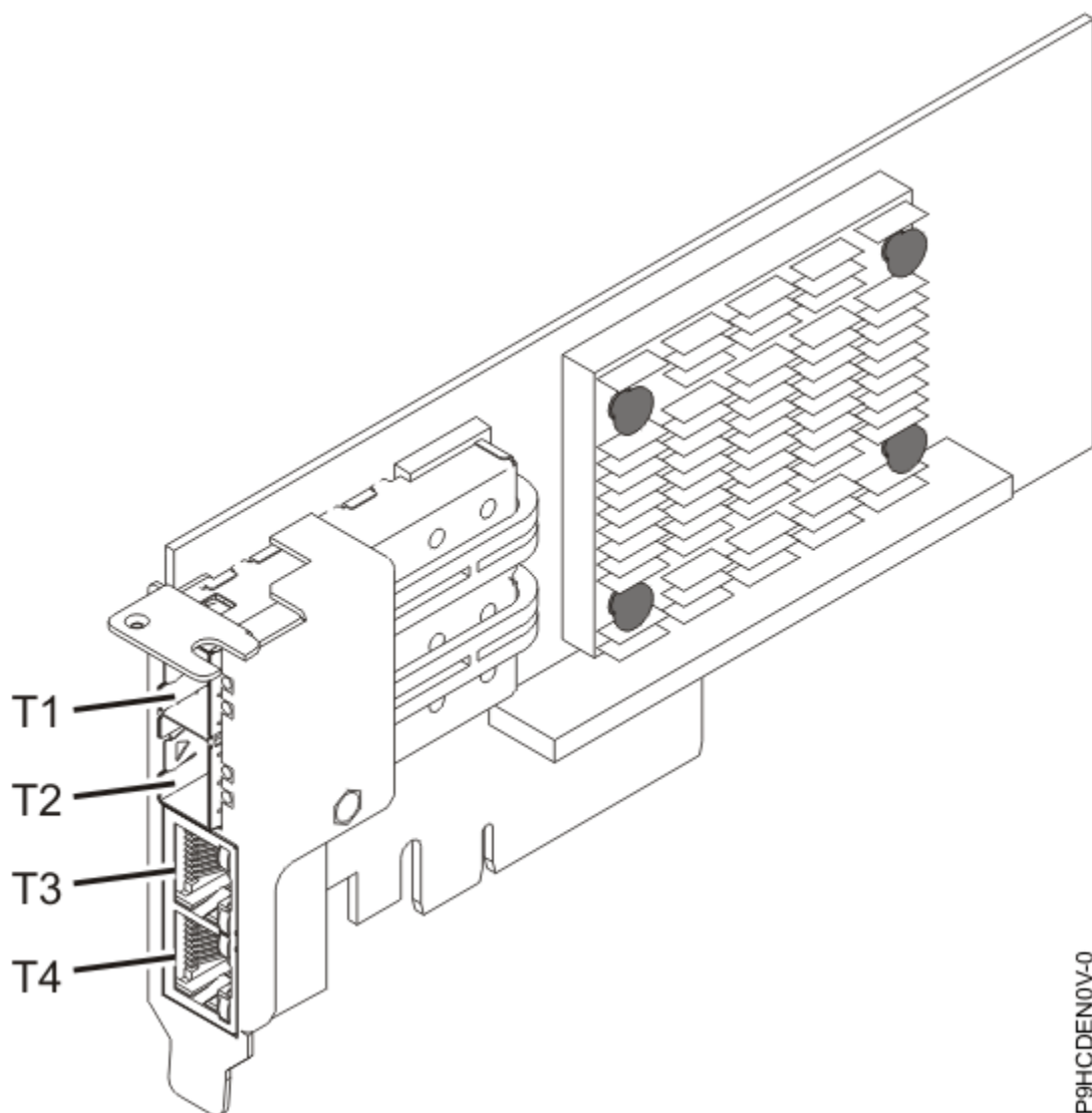
Figure 30. Carte PCIe2 LP 4 ports (10 Gb + 1 GbE) cuivre SFP+RJ45
