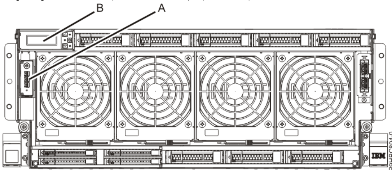
Figura 1. Paneles de control
