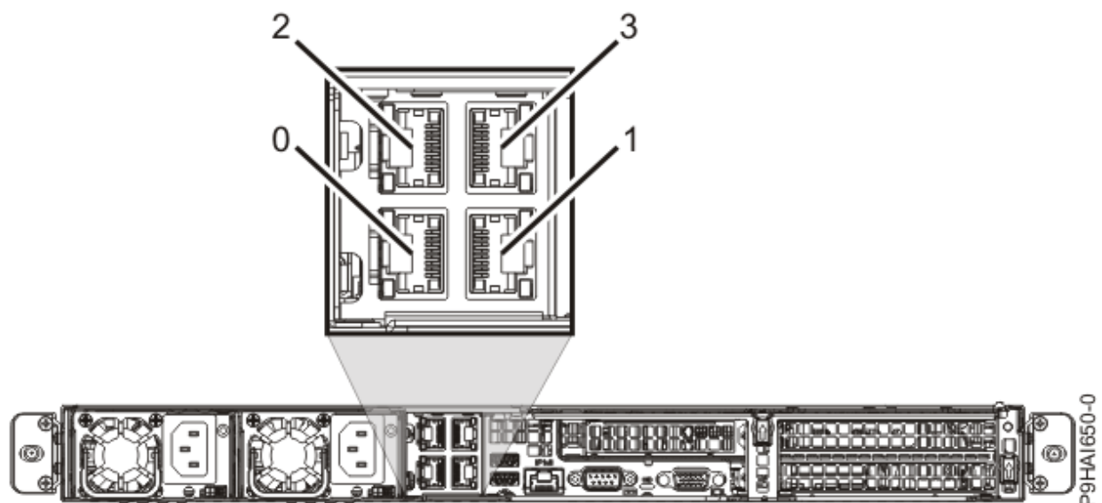
Figura 8. puertos Ethernet
