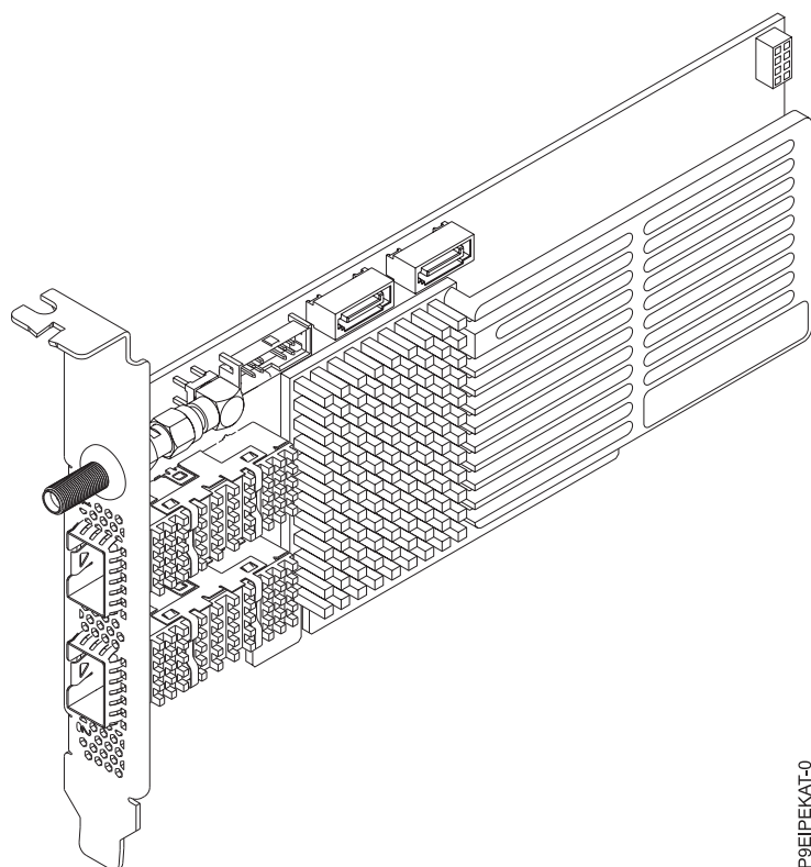
Figura 38. Kit Dev PCIe4 x8 AlphaData ADM-PCIE-9V3 CAPI2.0 FPGA (Xilinx VU3P)
