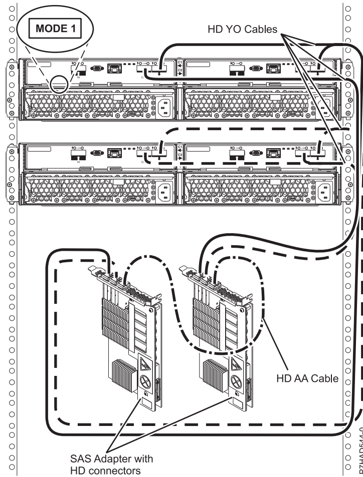
Figure 86. Mode 1 connection of two 5887 enclosures by using HD connectors to two PCIe2 SAS adapters
