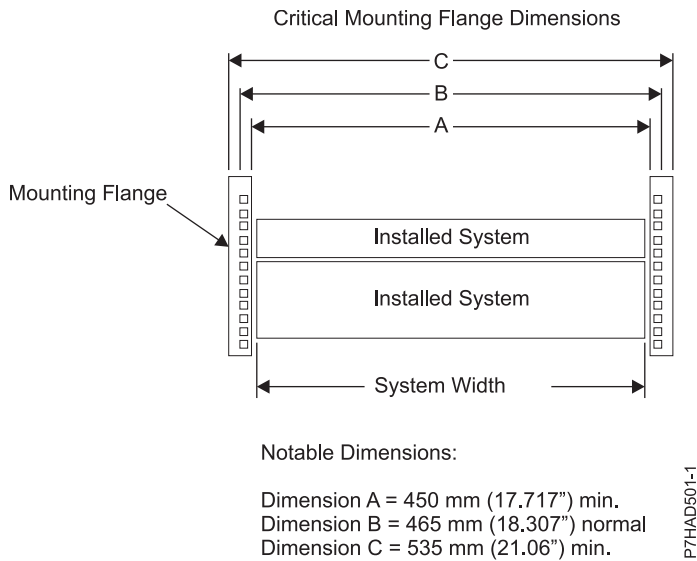
Figure 47. Critical mounting flange dimensions
