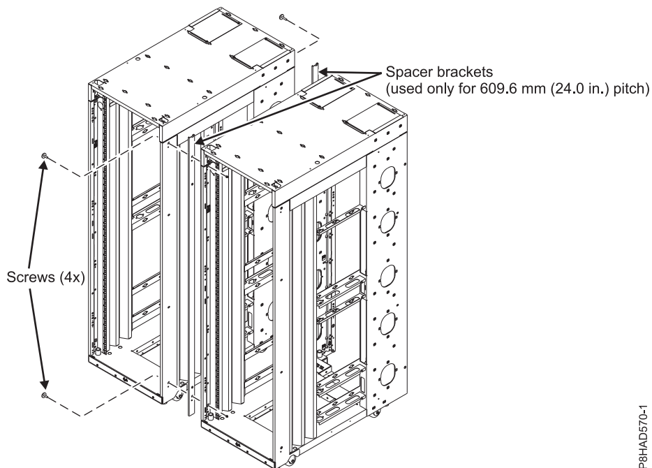
Figure 40. Attaching multiple racks with spacer brackets
