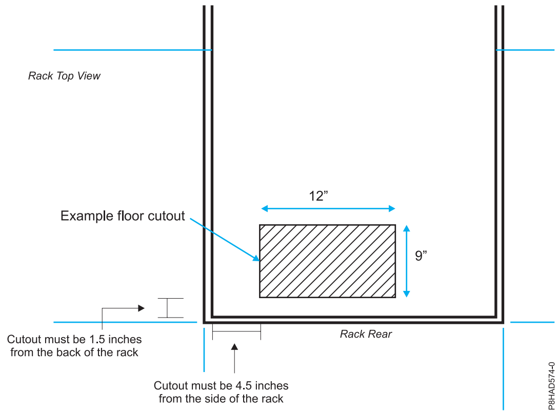
Figure 35. Floor cutout
