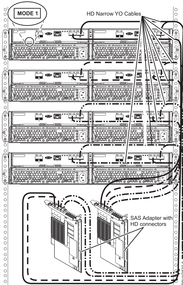
Figure 92. Mode 1 connection of four 5887 enclosures to two PCIe3 SAS adapters with HD narrow connectors.
