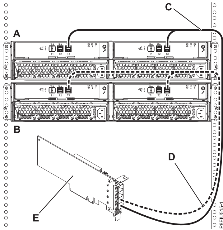
Figure 96. Mode 1 connection of two ESLL or ESLS storage enclosures by using YO12 cables to a single SAS adapter
