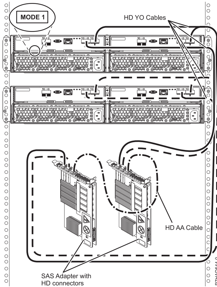
Figure 86. Mode 1 connection of two 5887 enclosures by using HD connectors to two PCIe2 SAS adapters
