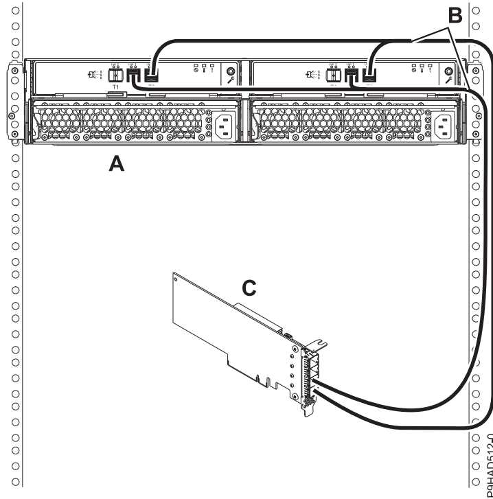
Figure 100. Mode 2 connection of ESLL or ESLS storage enclosure by using YO12 cables to a single SAS adapter
