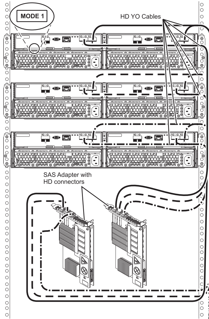
Figure 87. Mode 1 connection of three 5887 enclosures to two PCIe2 SAS adapters with HD connectors
