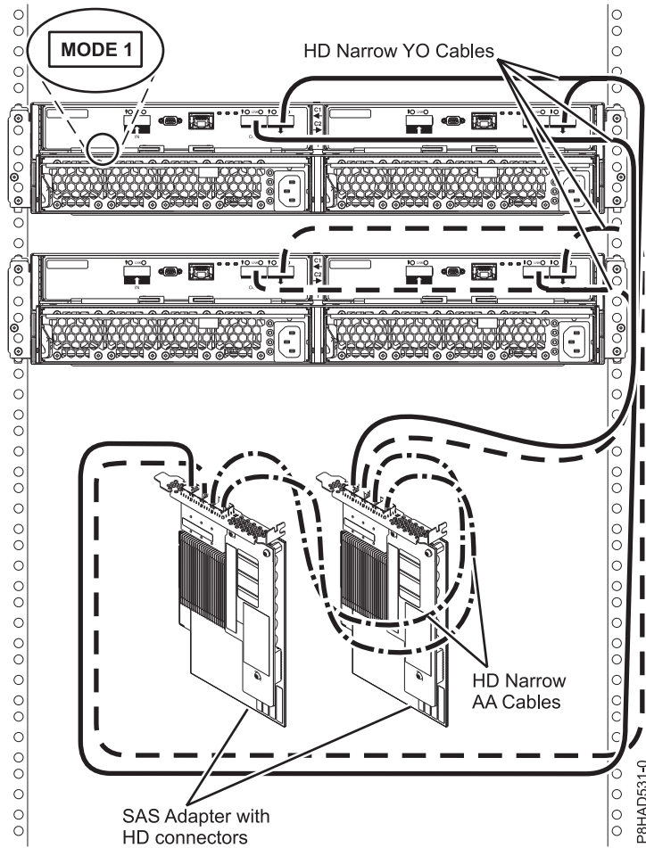
Figure 90. Mode 1 connection of two 5887 enclosures to two PCIe3 SAS adapters with HD narrow connectors.
