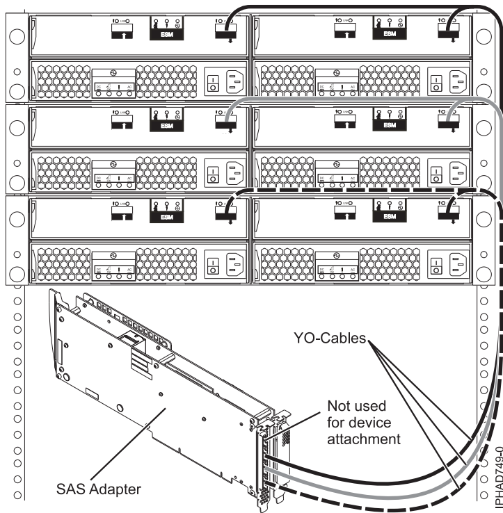
Figure 63. Tri-port SAS adapter to disk expansion drawers
