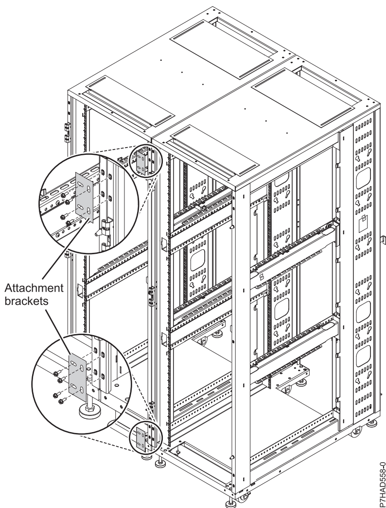
Figure 31. Attachment brackets
