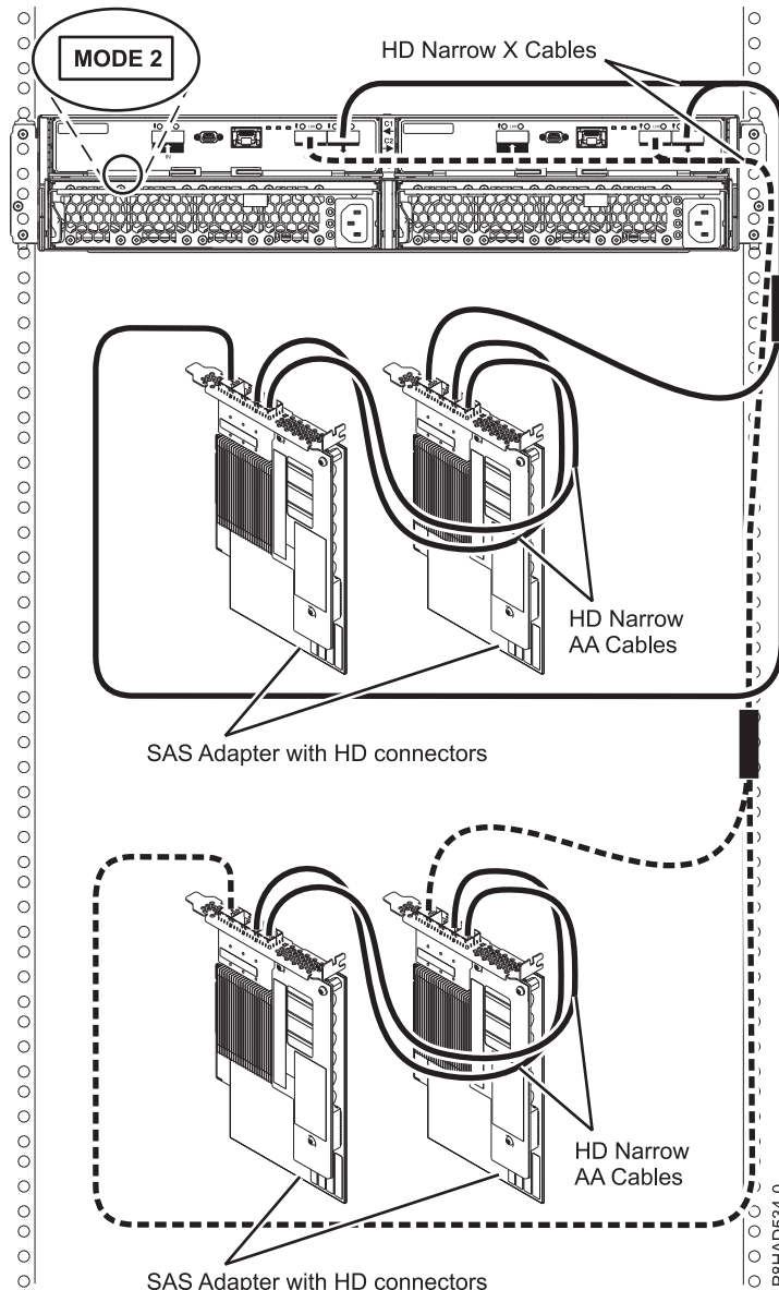
Figure 93. Mode 2 connection of a 5887 enclosure to two pairs of PCIe3 SAS adapters with HD narrow connectors.
