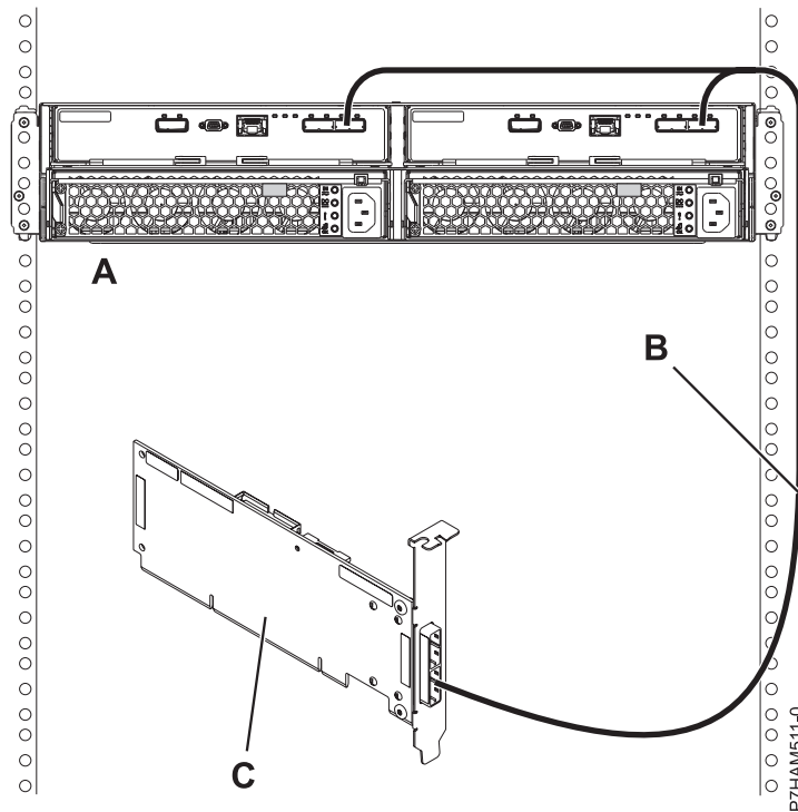
Figure 78. Mode 1 connection of a 5887 enclosure by using a YO cable to a single SAS adapter
