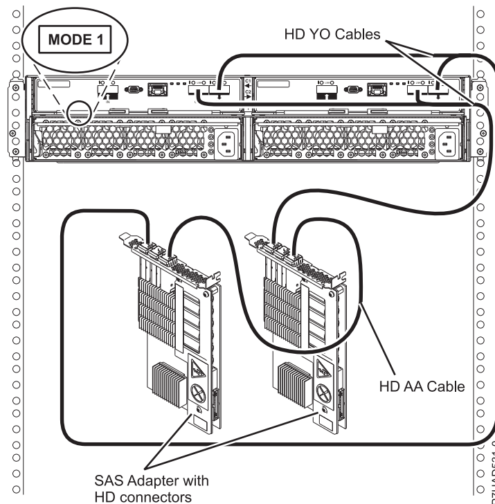
Figure 85. Mode 1 connection of a 5887 enclosure to two PCIe2 SAS adapters with HD connectors
