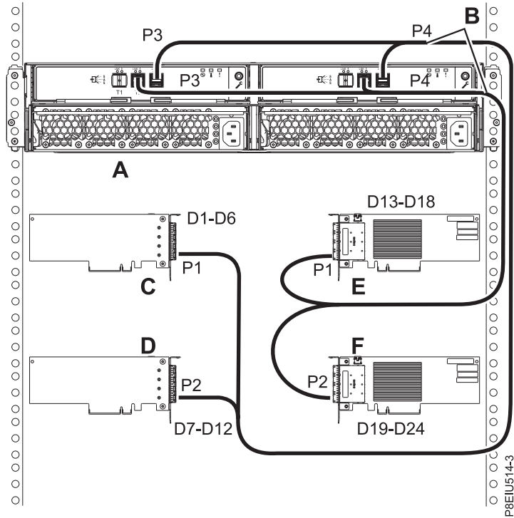
Figure 102. Mode 4 connection of one ESLL or ESLS storage enclosure by using X12 cables to four independent SAS adapters
