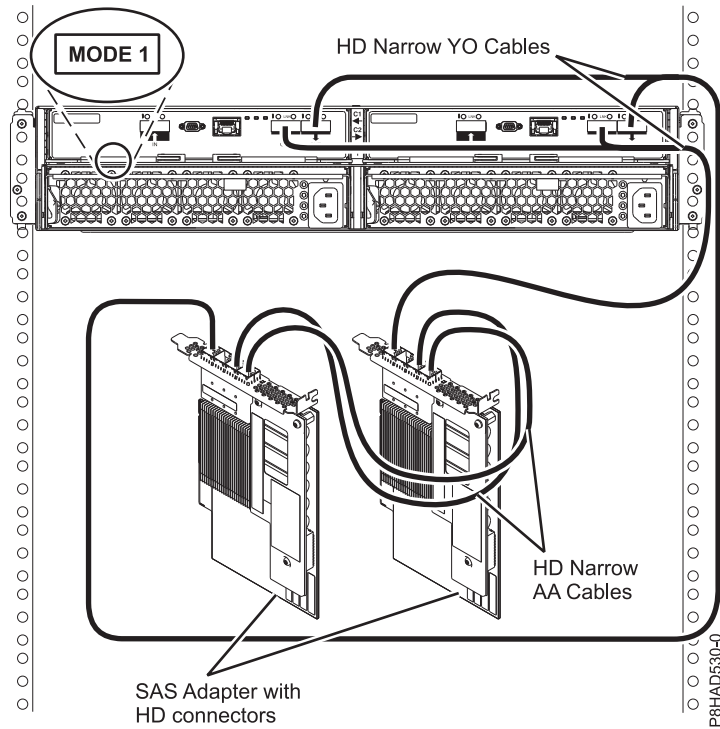
Figure 89. Mode 1 connection of a 5887 enclosure to two PCIe3 SAS adapters with HD narrow connectors.
