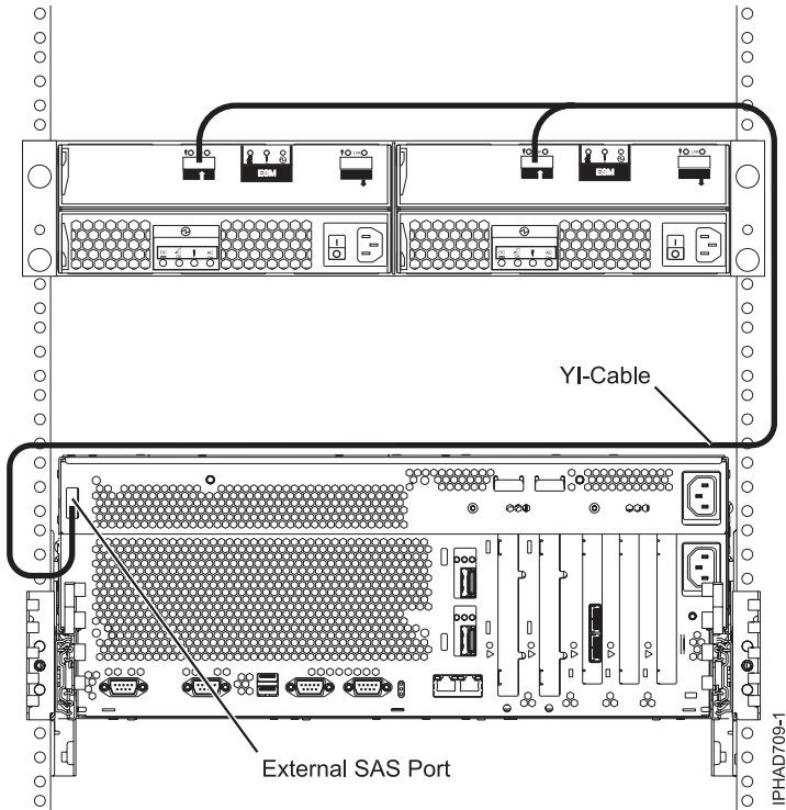
Figure 66. System external SAS adapter port to a disk expansion drawer
