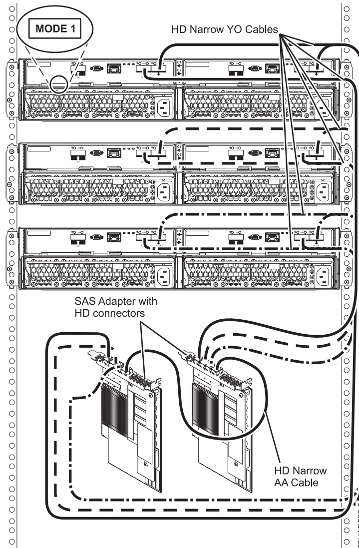
Figure 91. Mode 1 connection of three 5887 enclosures to two PCIe3 SAS adapters with HD narrow connectors.
