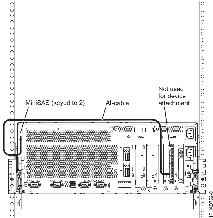
Figure 68. FC5904 or FC5908 adapter attached to disk expansion drawers
