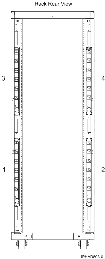
Figure 50. Power distribution unit vertical locations
