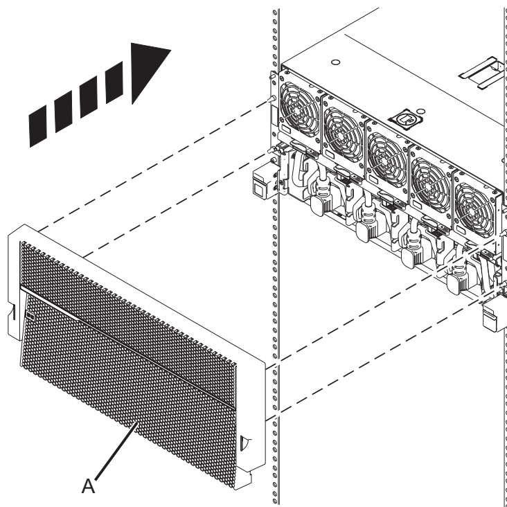
Figura 16. Instalar a tampa frontal
