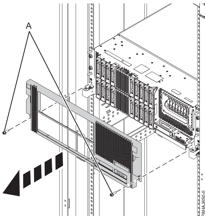
Figura 56. Remover a tampa frontal
