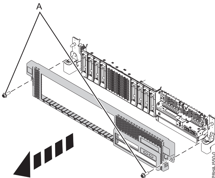
Figura 55. Remover a tampa frontal
