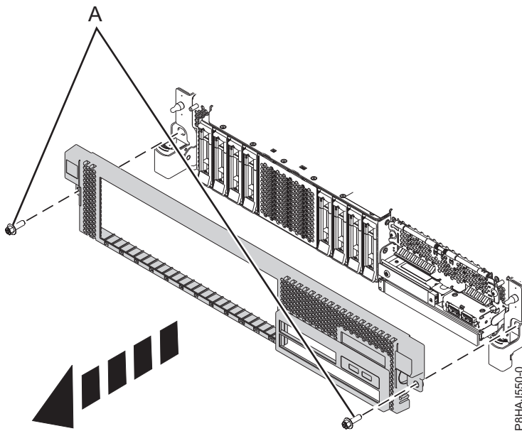
Figura 95. Remover a tampa frontal
