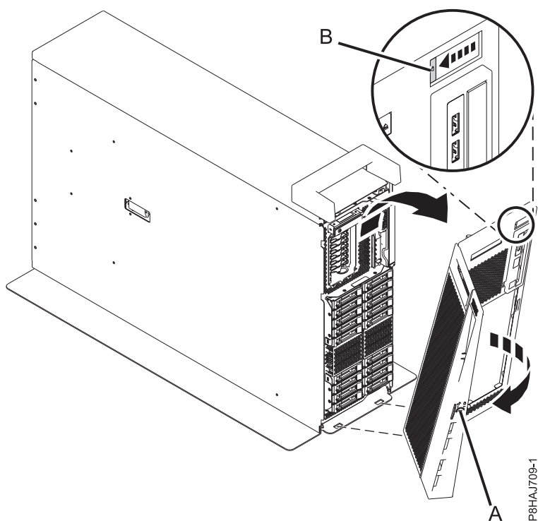
Figura 97. Remover a tampa frontal
