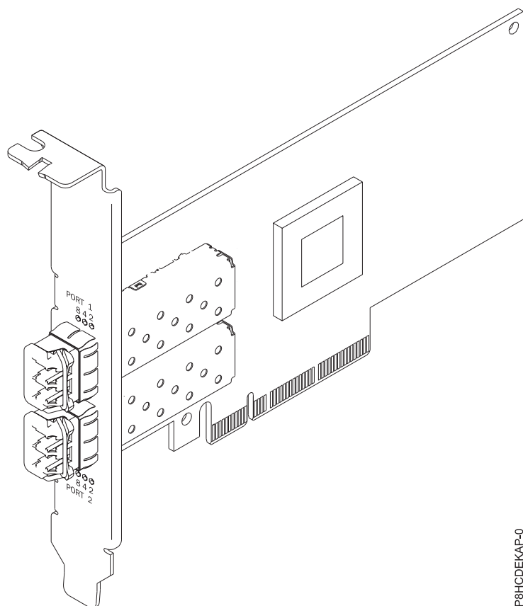
Figura 38. Placa Fibre Channel QLogic Low-profile Padrão 8 Gb
