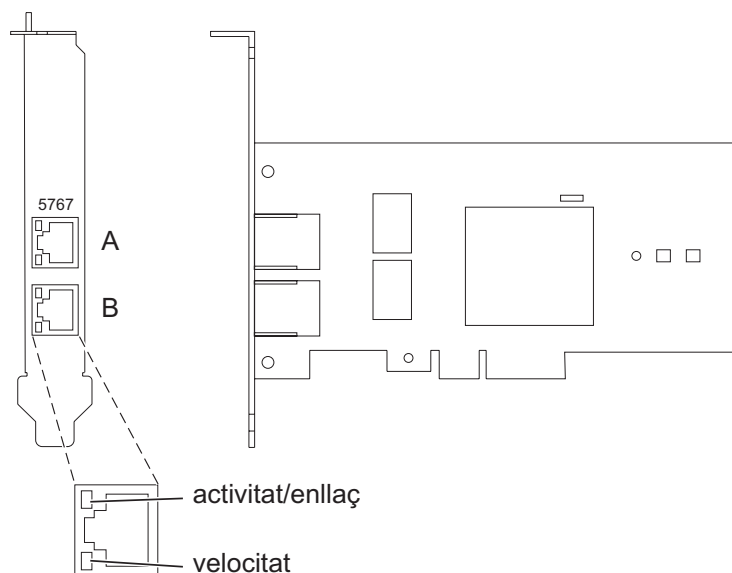
Figura 24. Adaptador 10/100/1000 Base-TX Ethernet PCI Express de 2 ports
