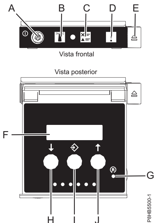
Figura 13. Panell de control
