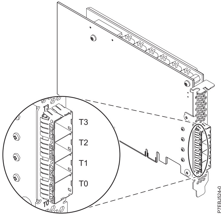
Figure 24. CCIN 57CE PCIe3 12 GB cache RAID SAS adapter Quad-port 6 Gb x8
