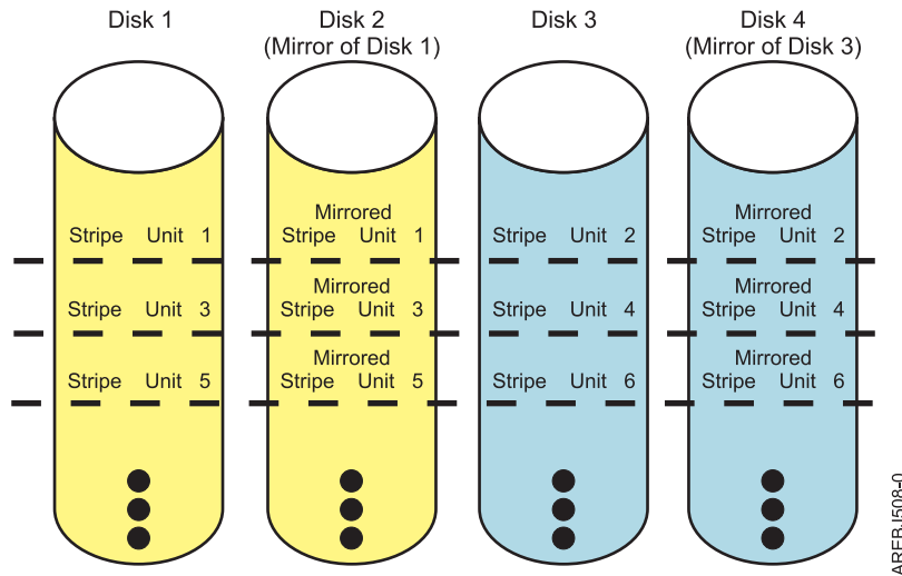
Figure 30. RAID 10
