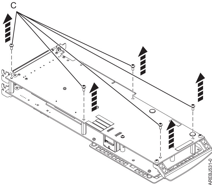
Figure 41. Location of screws on the 572F/575C card set adapter
