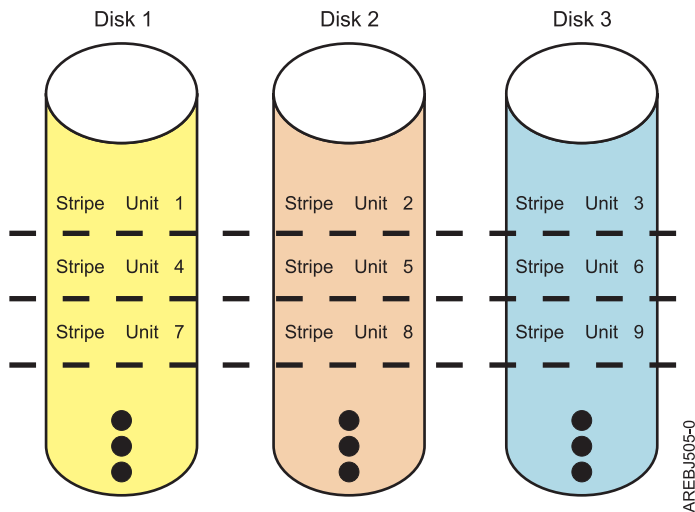
Figure 27. RAID 0
