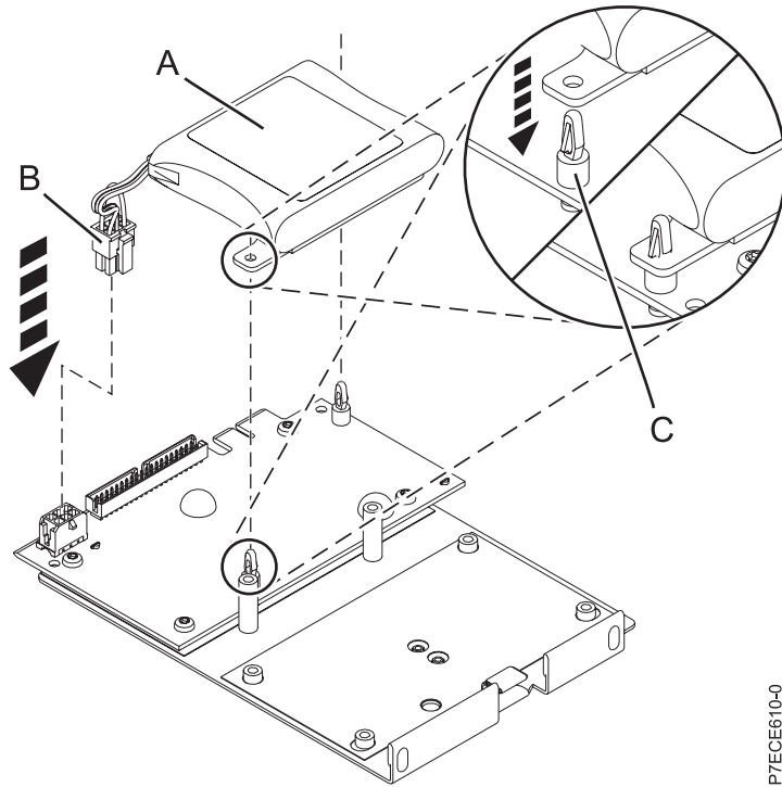
Figure 39. Replacing the cache battery
