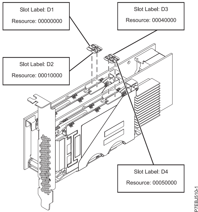
Figure 52. SAS resource locations for CCIN 57CD PCIe SAS RAID and 3 Gb x8 SSD Adapter
