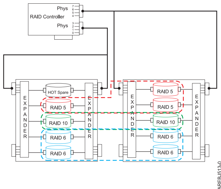
Figure 26. Disk array configuration
