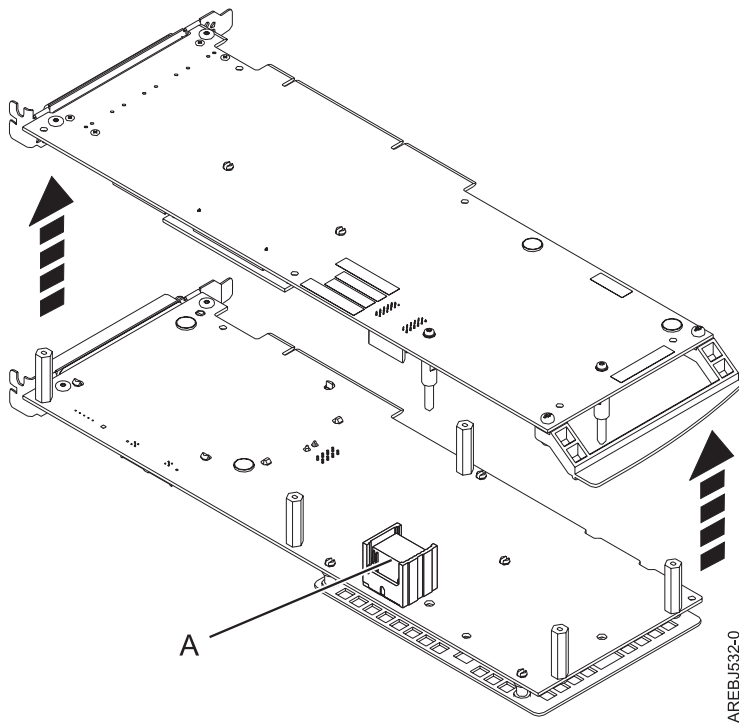
Figure 42. Location of interconnect connector on the 572F/575C card set adapter
