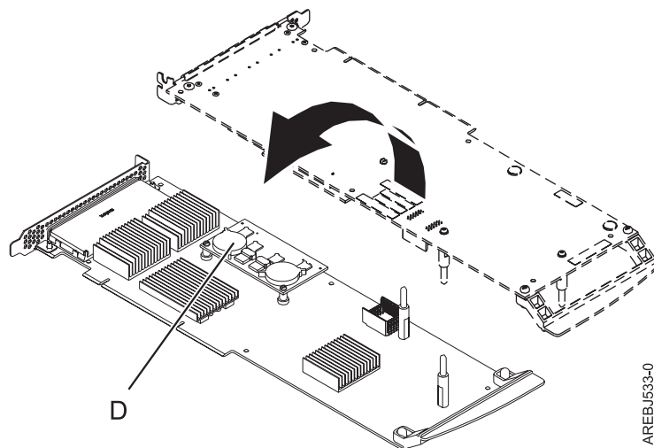
Figure 43. Cache directory card
