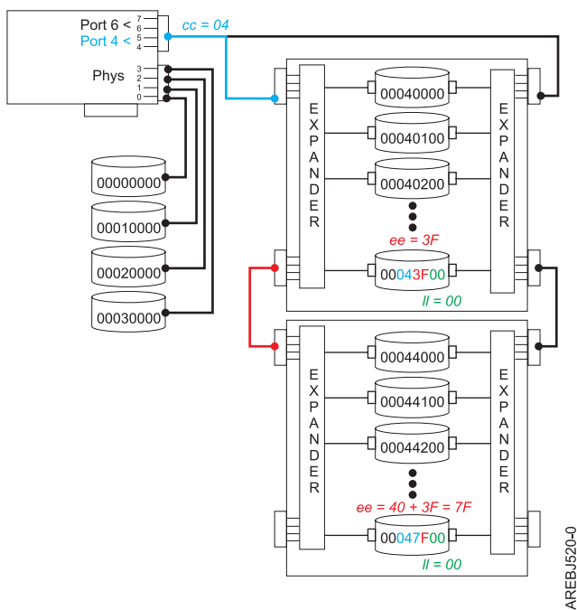
Figure 51. Example SAS subsystem resource locations
