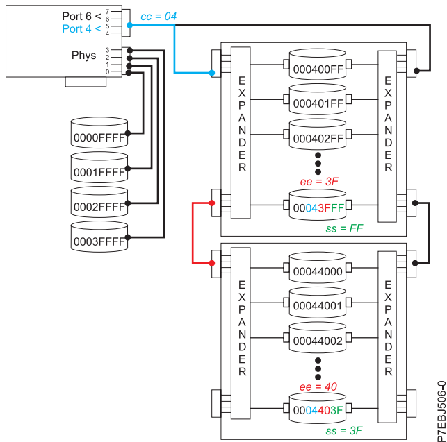
Figure 53. Example PCIe2 or PCIe3 SAS subsystem resource locations
