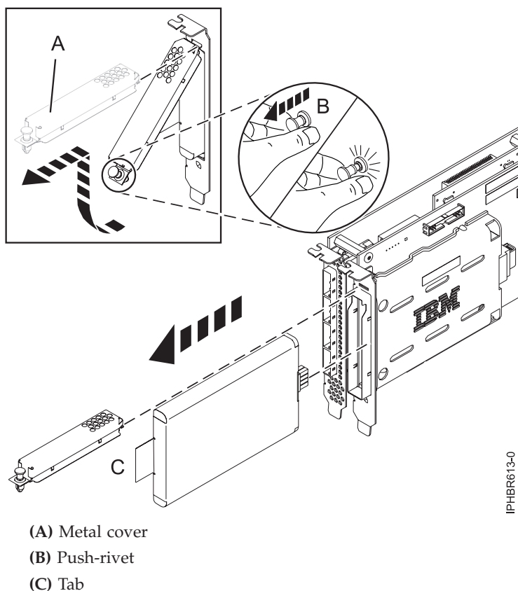
Figure 34. Replacing the 572F/575C cache battery
