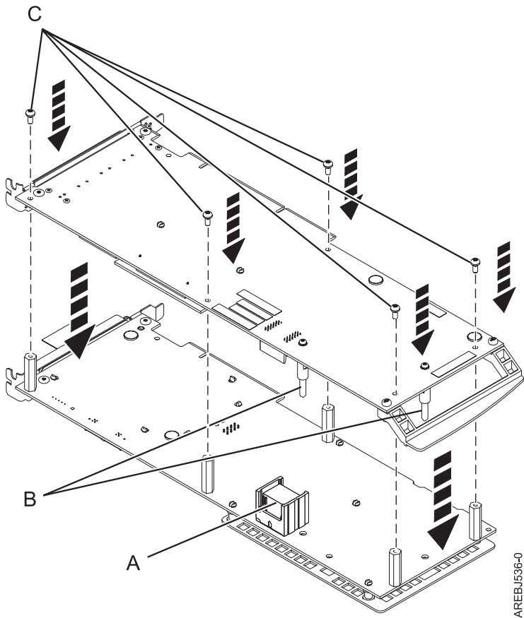
Figure 45. Reassembling the cards
