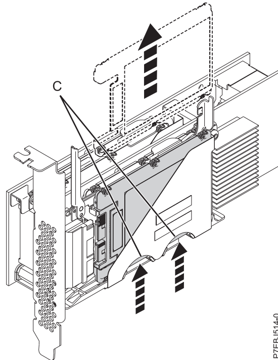
Figure 50. Pushing the SSD that is being replaced
