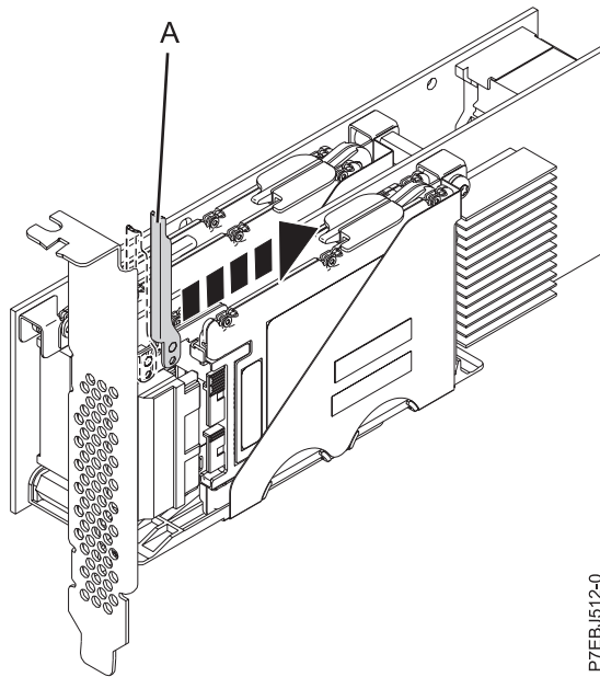
Figure 48. Pushing the lever away from the adapter tailstock
