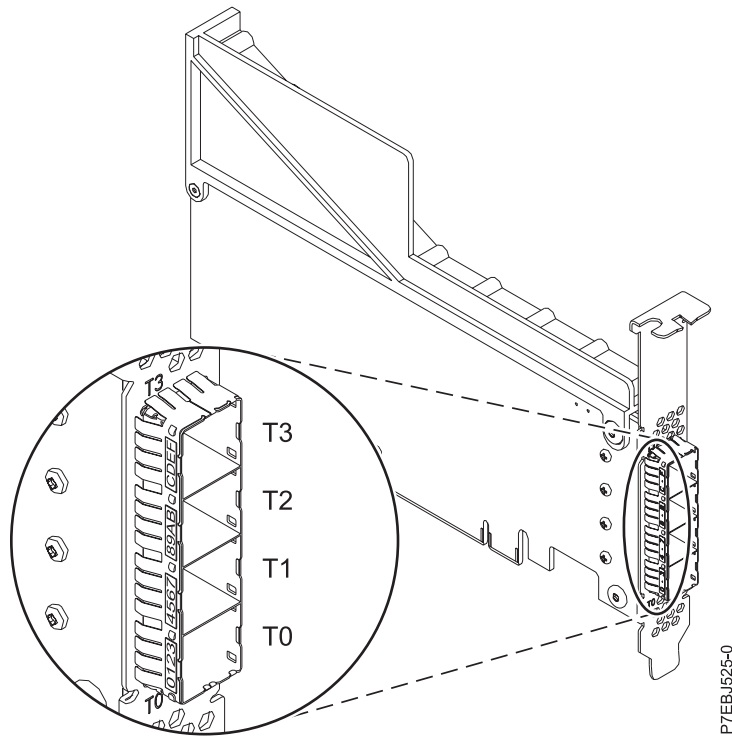
Figure 22. CCIN 57B4 PCIe3 RAID SAS adapter Quad-port 6 Gb x8, two units
