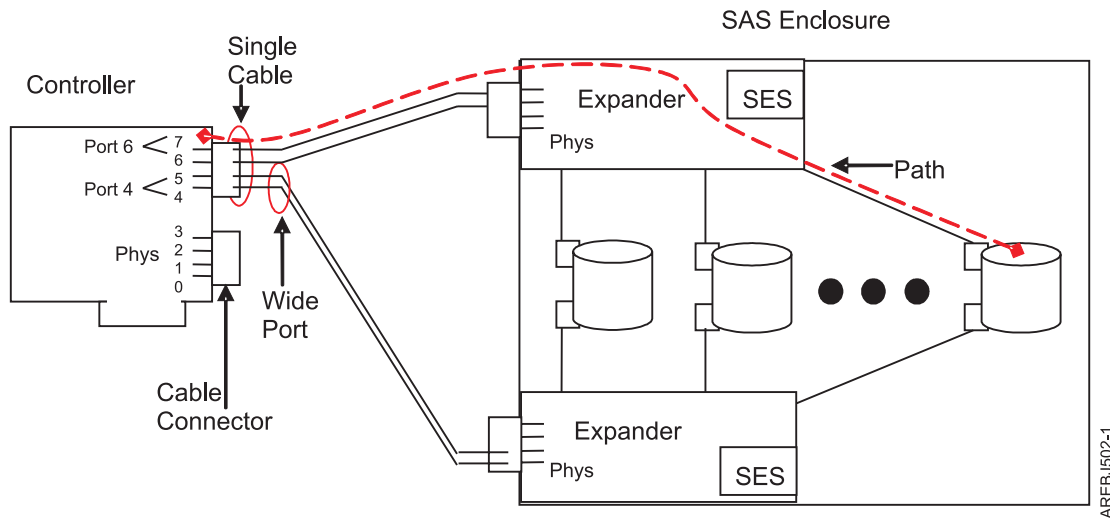
Figure 25. Example SAS subsystem
