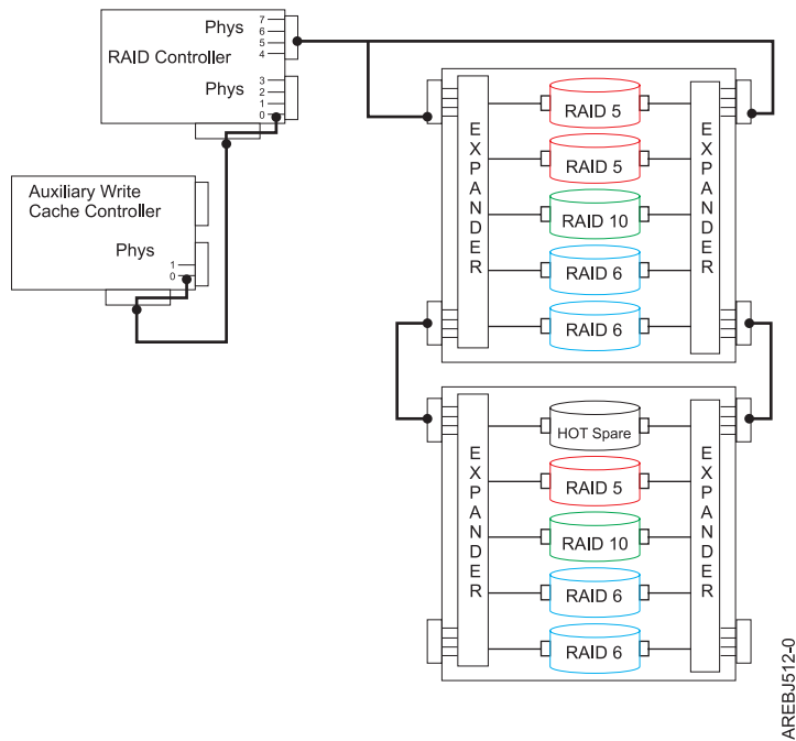
Figure 31. Example RAID and AWC controller configuration
