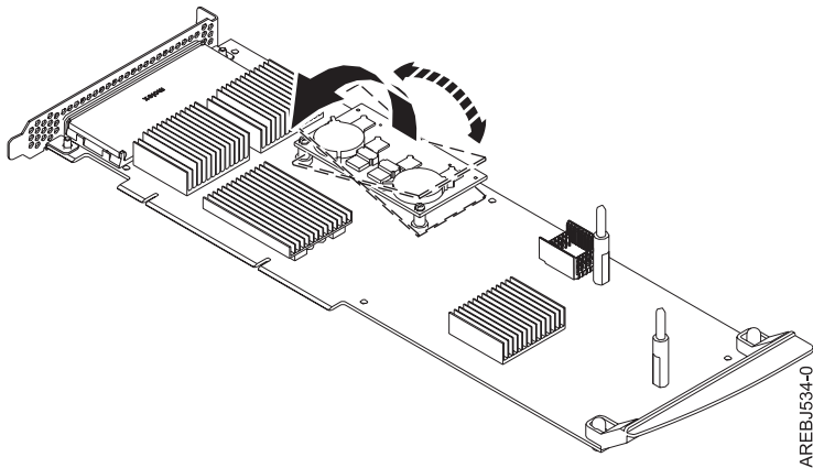
Figure 44. Unseating the connector
