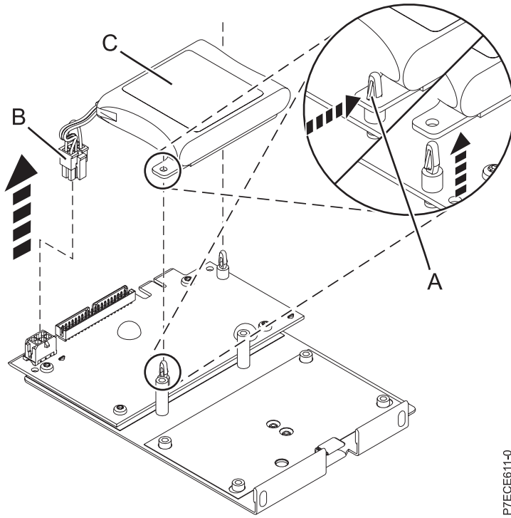
Figure 38. Removing the cache battery
