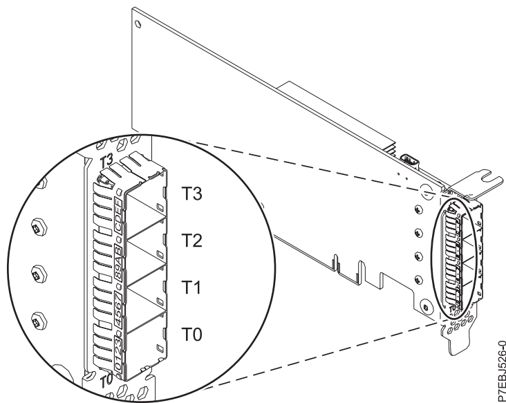
Figure 23. CCIN 57B4 PCIe3 RAID SAS adapter Quad-port 6 Gb x8, four units
