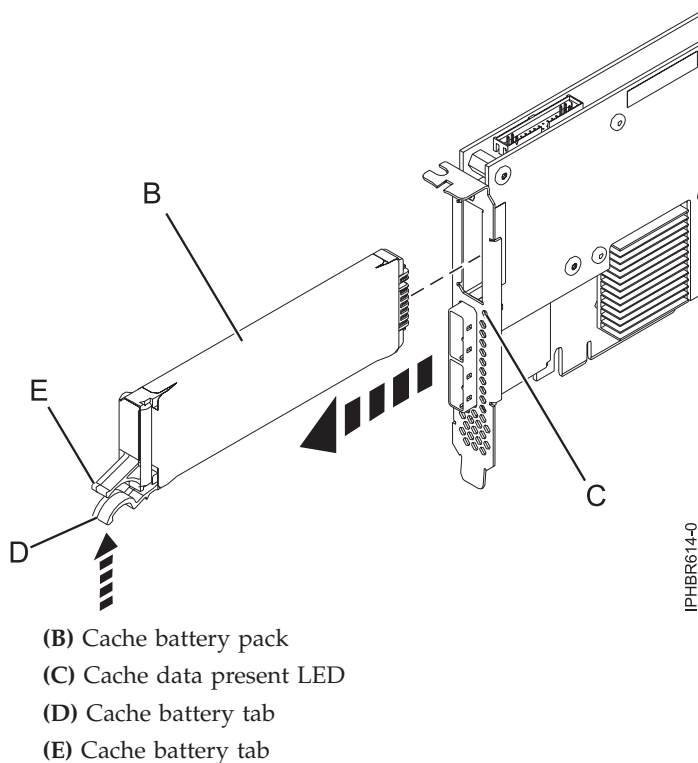
Figure 35. Replacing the 574E cache battery
