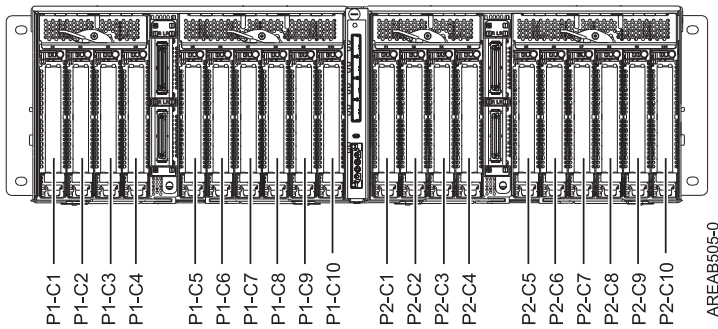
Figure 2. Rear view
