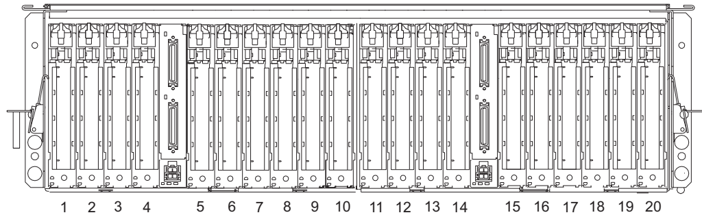
Figure 1. Expansion unit rear view with numbered slots
