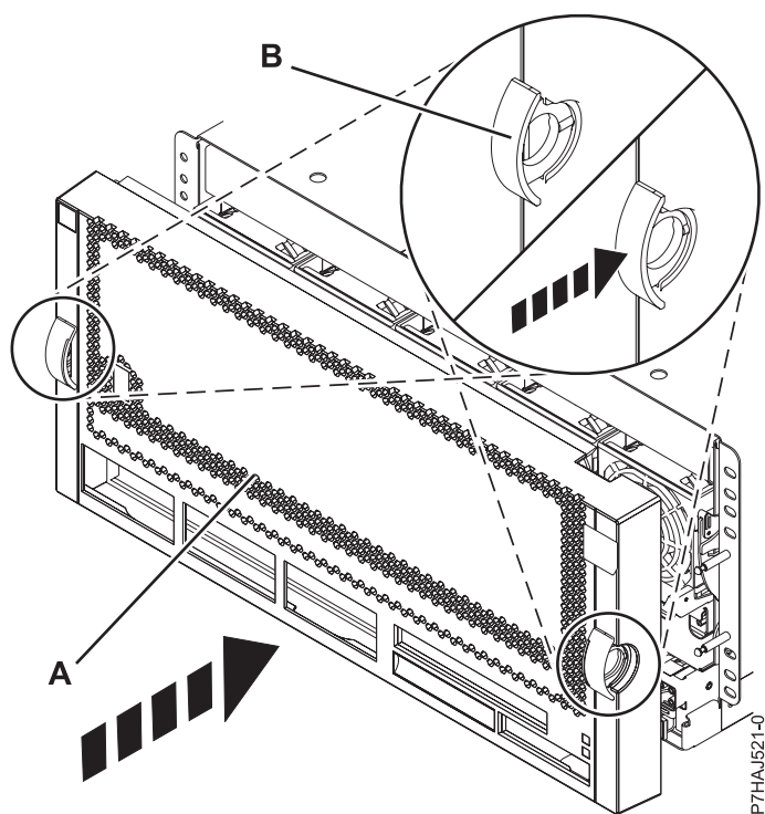
Figura 7. Instalar a tampa frontal
