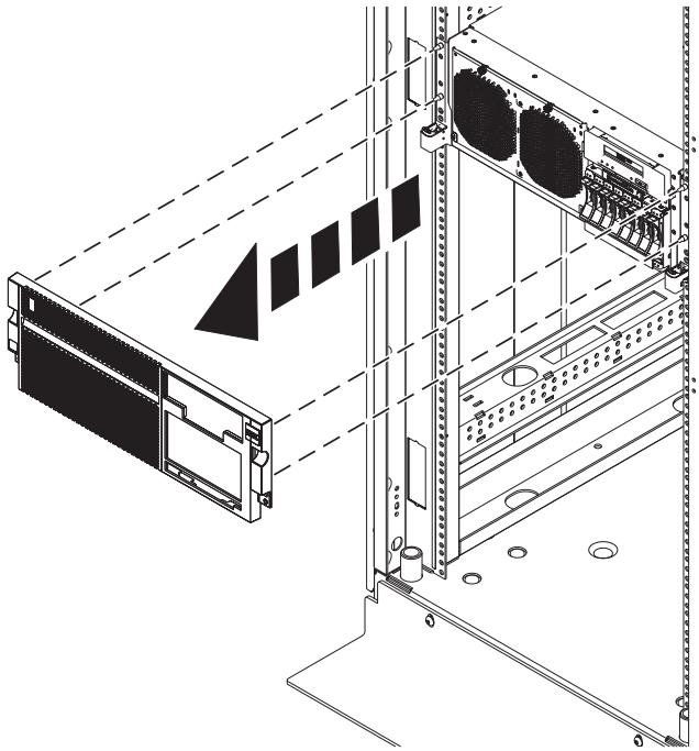
Figura 22. Remover a tampa frontal
