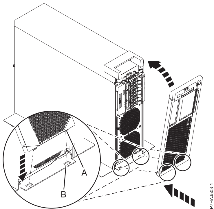
Figura 25. Instalar a tampa frontal
