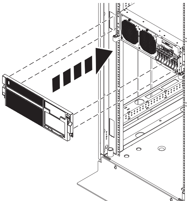
Figura 24. Remover a tampa frontal
