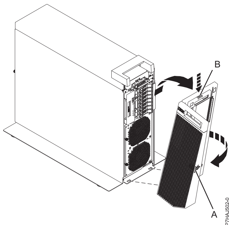
Figura 23. Remover a tampa frontal
