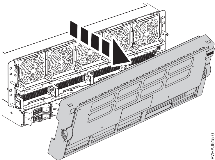
Figura 12. Remover a tampa
